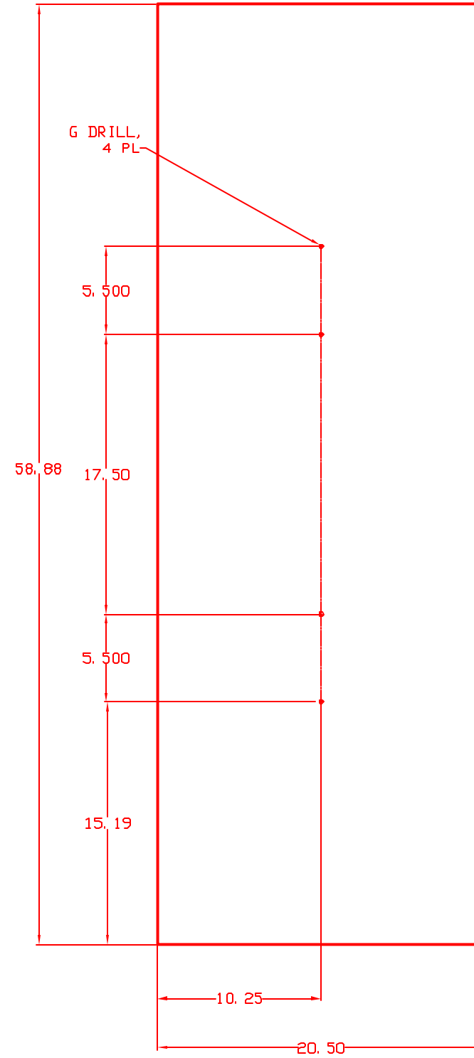
-2 21X59 LID MAT'L: 6061-T6 ALUMINUM; 7 REQ'D.
