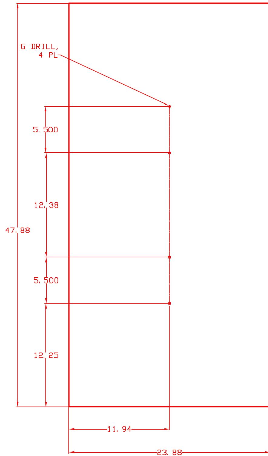
-1 24x48 LID MAT'L: 6061-T6 ALUMINUM; 6 REQ'D.
