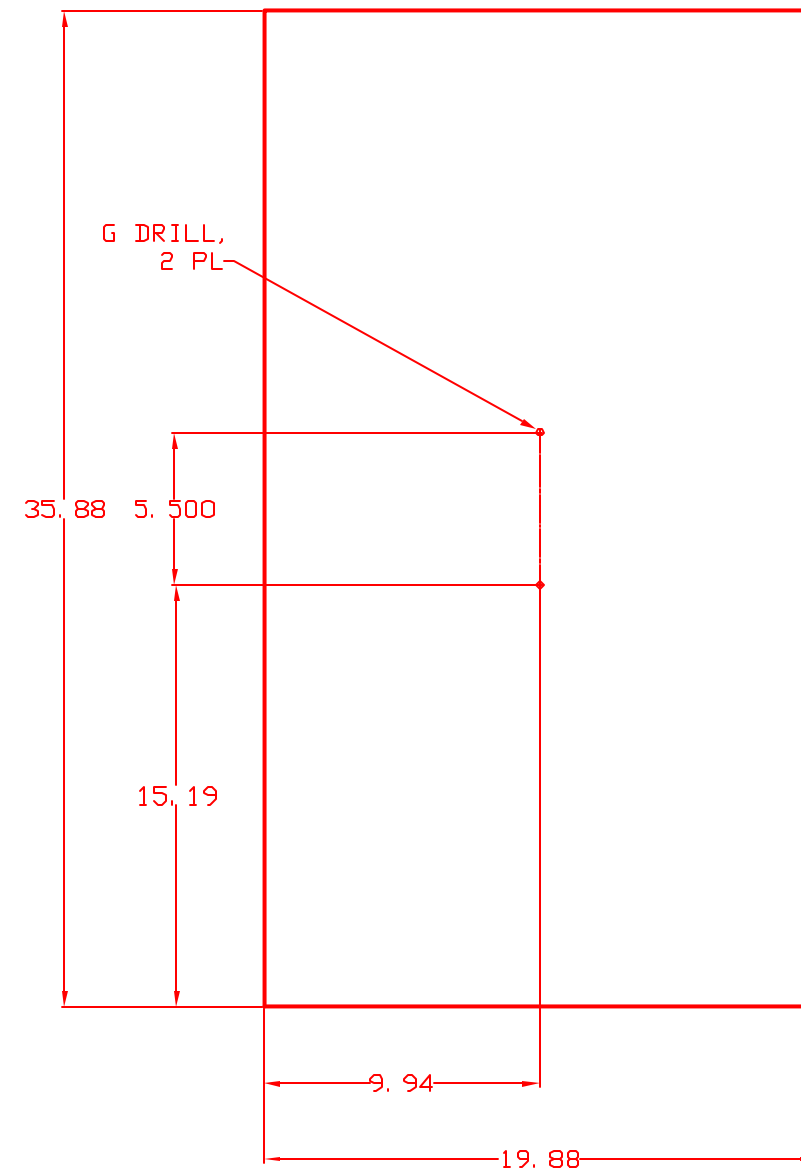
-2 20x36 LID MAT'L: 6061-T6 ALUMINUM; 3 REQ'D.
