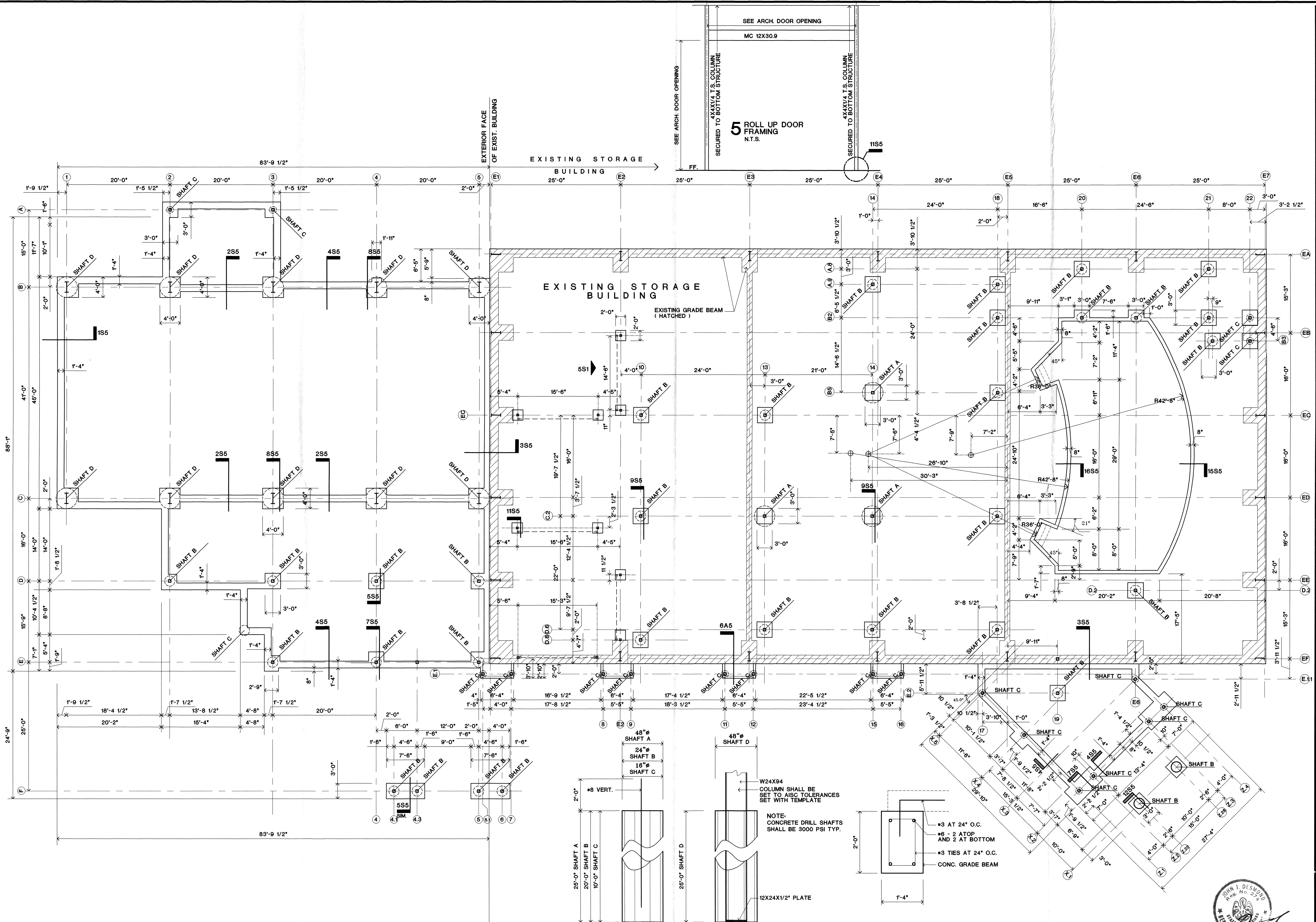
1 GRADE BEAM - DRILL SHAFTS PLAN 1/8" = 1'-0"
