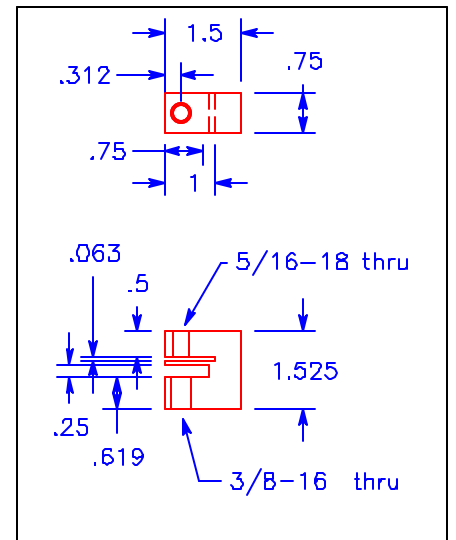
Lock Block
