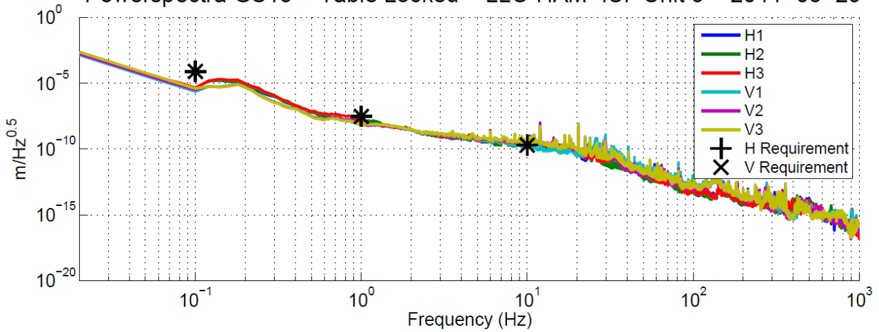
Powerspectra GS13 – Table Unlocked – LLO HAM-ISI-Unit 3 – 2011-03-25
