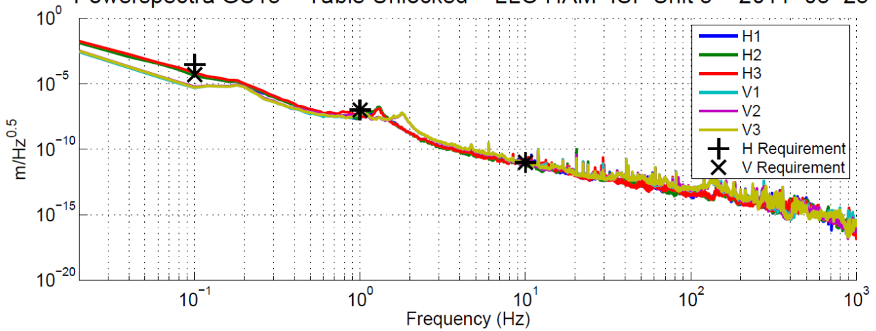
Figure – Power spectrum Calibrated GS13
