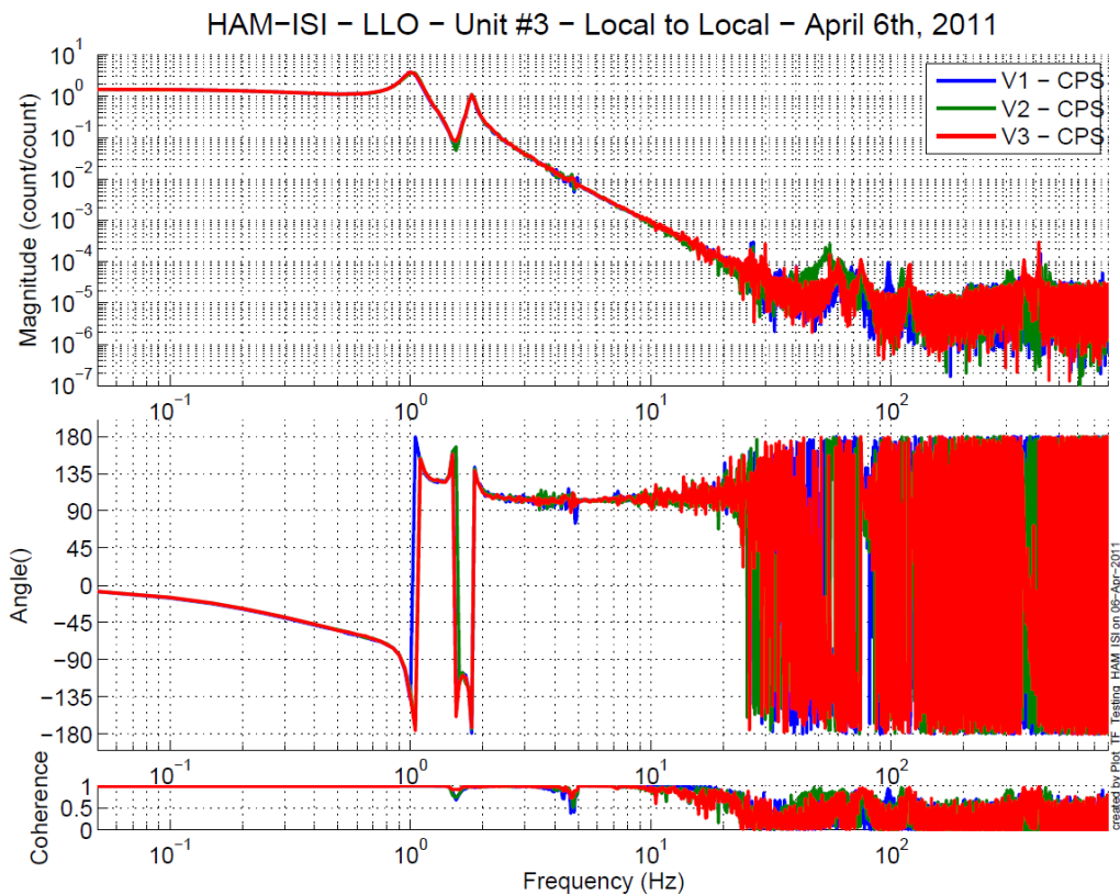
Figure - Local to Local Measurements – Vertical capacitive sensors
