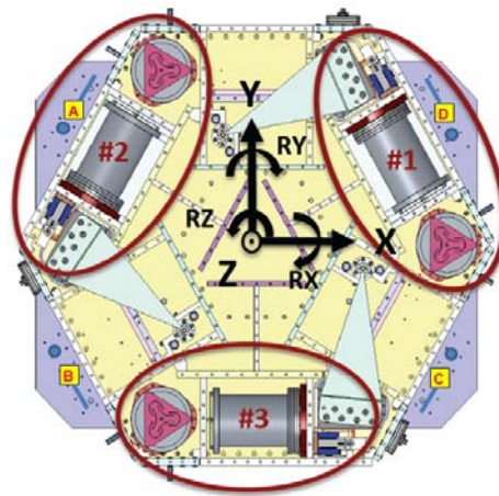
Figure - Top view of the HAM-ISI
