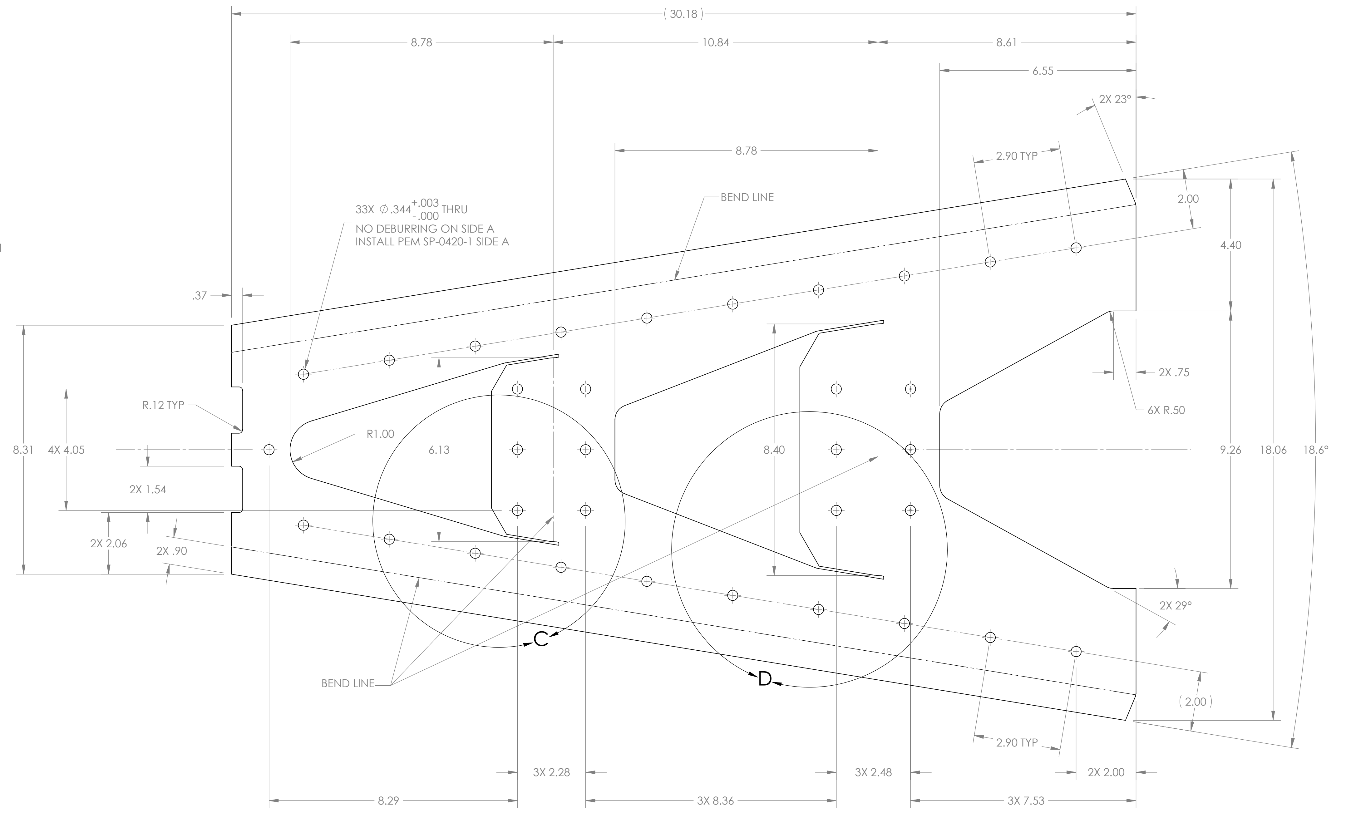
FLAT PATTERN
