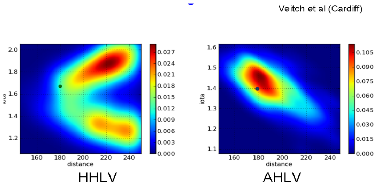
Figure 9 Two dimensional probability density contours for the model parameters of a binary neutron star system's luminosity distance and orbital inclination angle relative to the line of site in the two networks. The green dot shows the input value of the model parameter (iota is symmetric about \pi ). The solution using the HHLV network is bimodal. The degeneracy is broken in the AHLV network. The color coding indicates the amplitude of the probability density in units of 1/(\text{Mpc} \cdot \text{radian}) .
