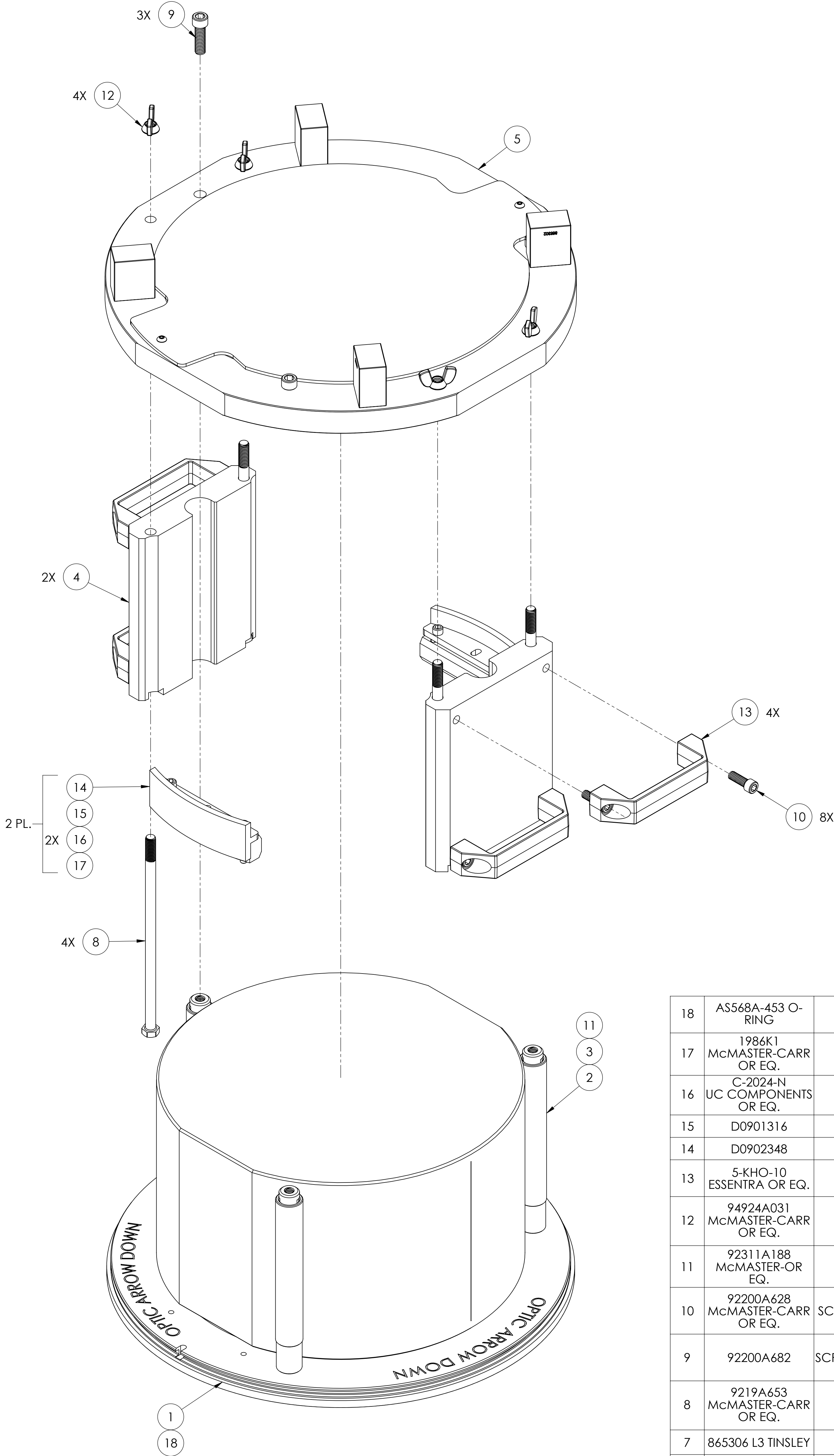
ISO VIEW
