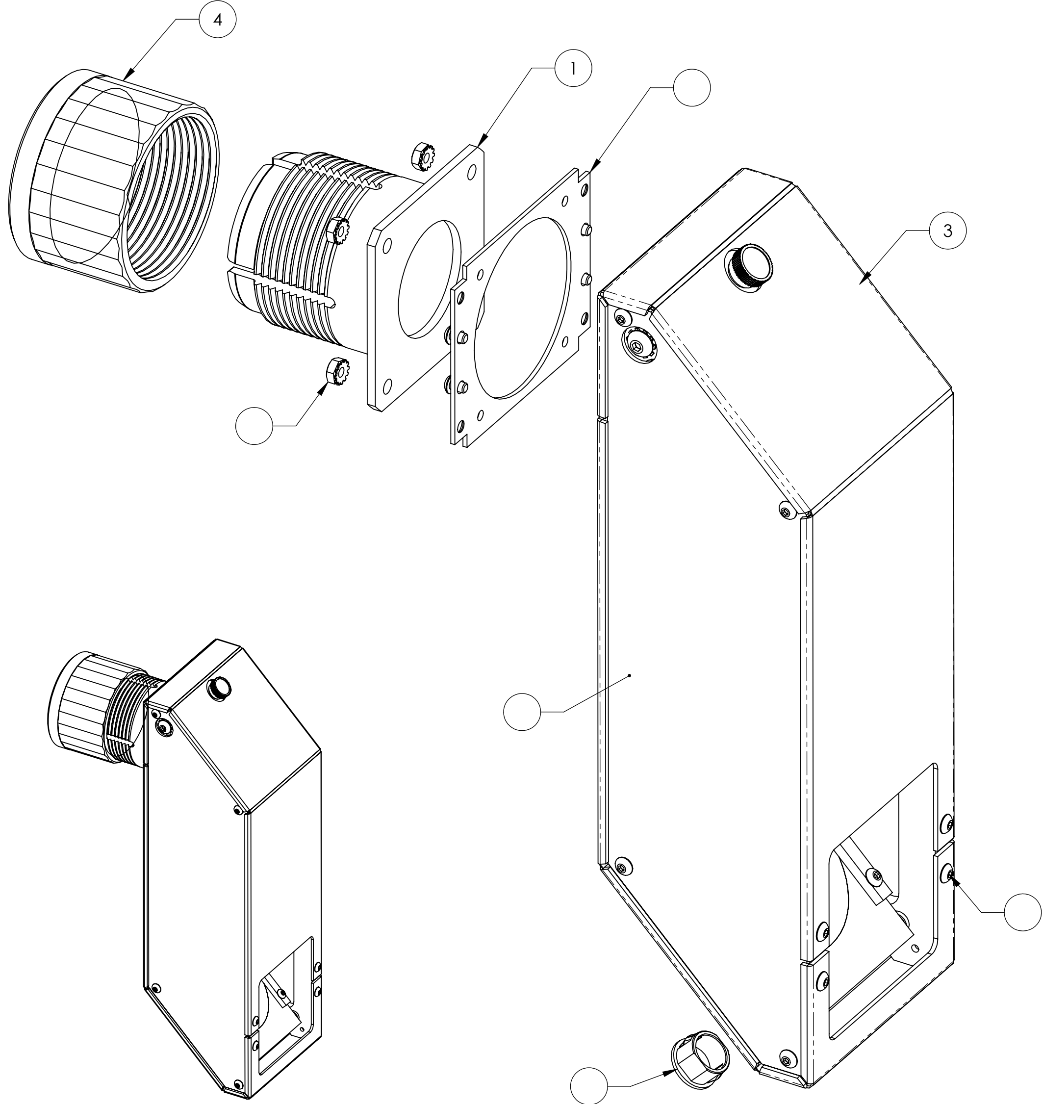
EXPLODED VIEW SCALE 1 : 1
