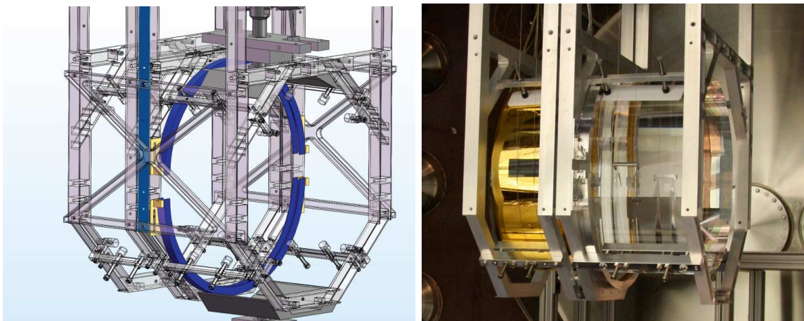
Figure 5.4: Rendering and image showing Advanced LIGO ring heater positioned 40 mm from the AR face of the test mass.
