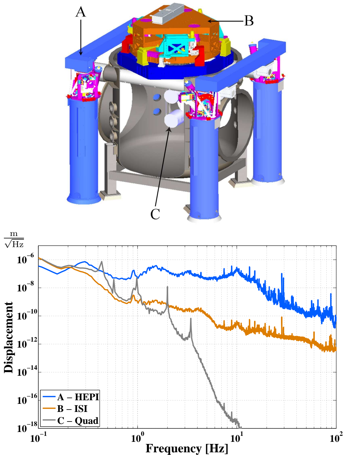
Figure 5.24: Top: Illustration showing the three layers of seismic isolation present in an AdvLIGO BSC chamber. A - The HEPI structure is shown in light blue with sensor-actuators in red/white/magenta. B - Above HEPI sits the ISI shown in dark blue (stage 0), cyan (stage 1) and orange (stage 2). C - Finally the quadruple pendulum (partially obscured) is fixed to stage 2 of the ISI. Bottom: Displacement noise after each stage of isolation at LASTI.
