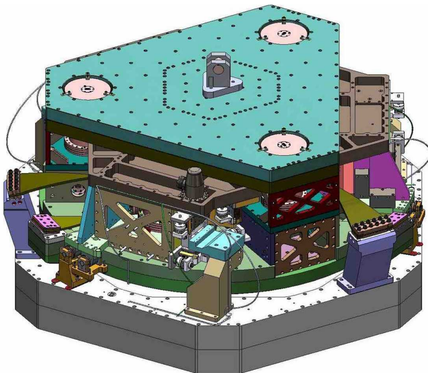
Figure 5.25: Rendering of redesigned BSC ISI. The ISI is rigidly fixed to HEPI and provides two stages of active isolation for the chamber’s optical table.
