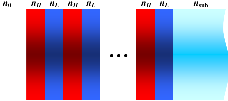
Figure 1.7: The optimal reflectivity Bragg mirror consists of alternating layers of high ( n_H ) and low ( n_L ) refractive index material where each layer has a thickness of \lambda/4 . The refractive indices of the substrate and surroundings are denoted by n_{\text{sub}} and n_0 respectively.
