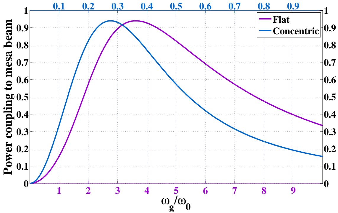
Figure 2.6: Power coupling |C|^2 between Gaussian and mesa beams as a function of Gaussian waist size \omega_g . The mesa beams are formed from minimal Gaussians of waist \omega_0 . The optimal coupling occurs when \omega_g \simeq 3.6\omega_0 for flat mesa beams and when \omega_g \simeq 0.28\omega_0 for concentric modes.
