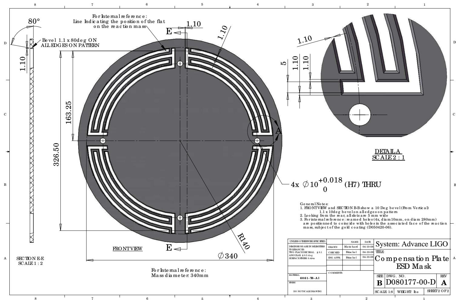
Figure B.2: Technical drawing of mask used in manufacture of LASTI prototype ESD (2 of 2). We assume perfect manufacturing and use the dimensions given in our model.
