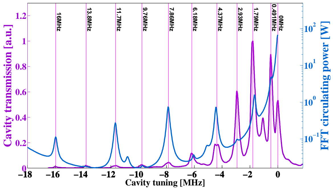
Figure 2.40: Comparison of experimental and numerical mesa beam transverse mode spectra. Notice that HOMs are not regularly spaced as with Gaussian resonators. The mesa spectrum can be compared to that shown in fig. 2.32 taken during a period of good alignment and input matching.
