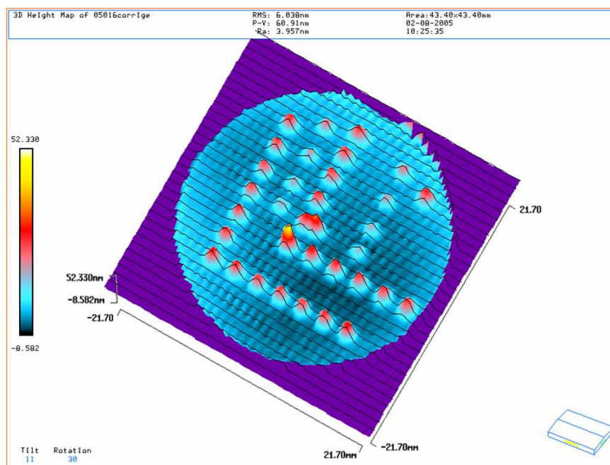
Figure 2.14: Calibration measurements for the second stage of mirror construction. Small amounts of material are deposited at regular intervals to allow characterisation of the robotic arm and corrective beam. Substrate diameter is 50 mm, the same as our experimental optic.
