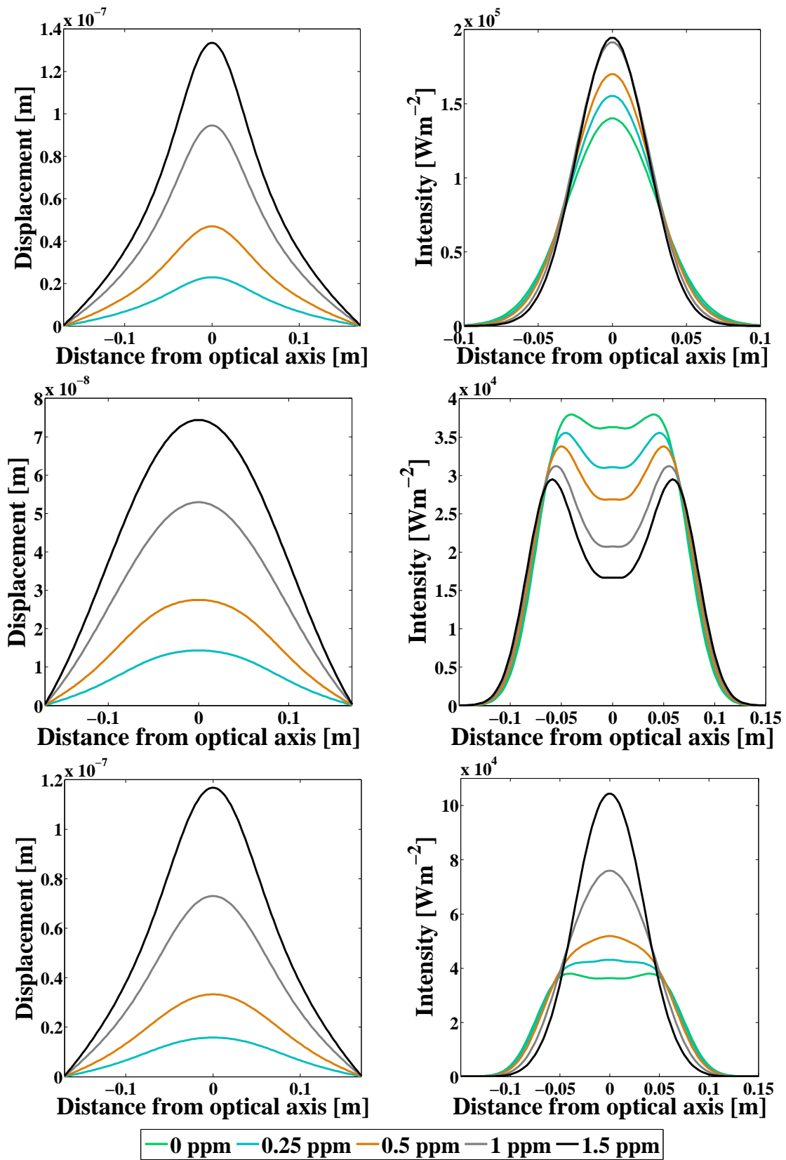
Figure 4.6: Thermoelastic deformation (left) and resonant mode shape (right) as a function of coating absorption. Top row: spherical cavity; middle row: flat mesa cavity; bottom row: concentric mesa cavity.
