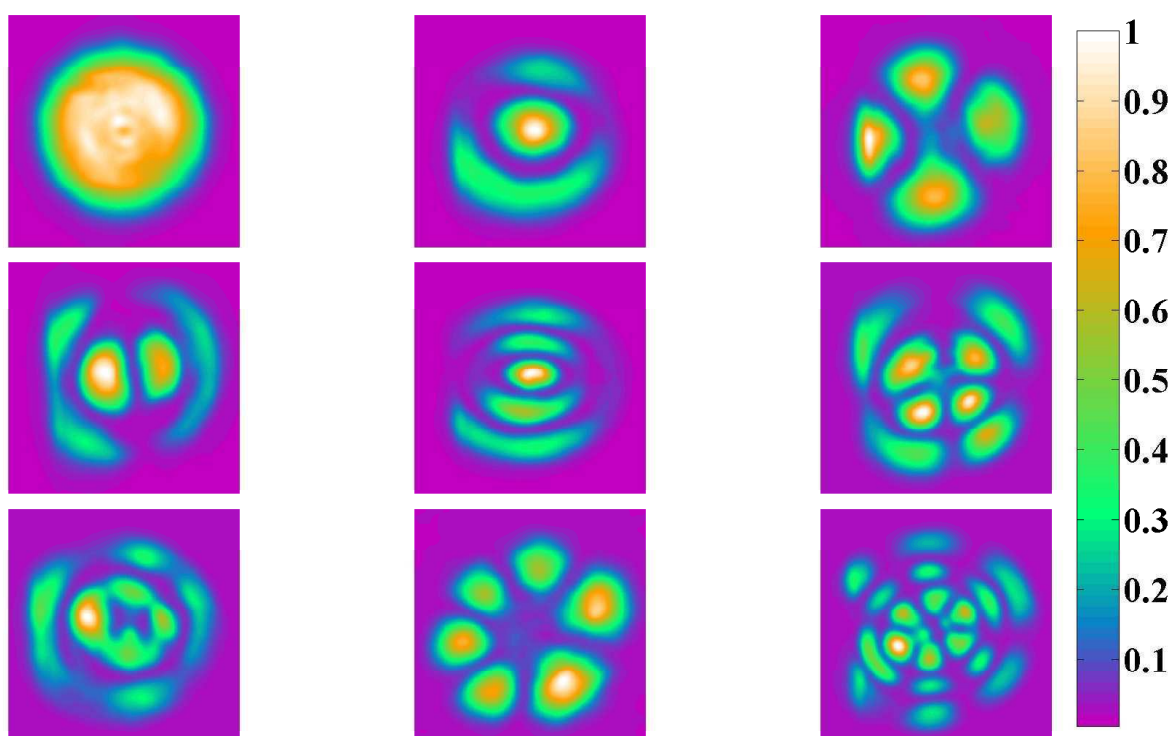
Figure 2.39: A selection of mesa beam transverse modes. These images were taken opportunistically during a period of poor input mode coupling efficiency. A complete catalogue of well formed higher order modes does not exist as efforts in this direction directly conflicted with our primary goal of maintaining good mode matching and alignment for the fundamental beam.
