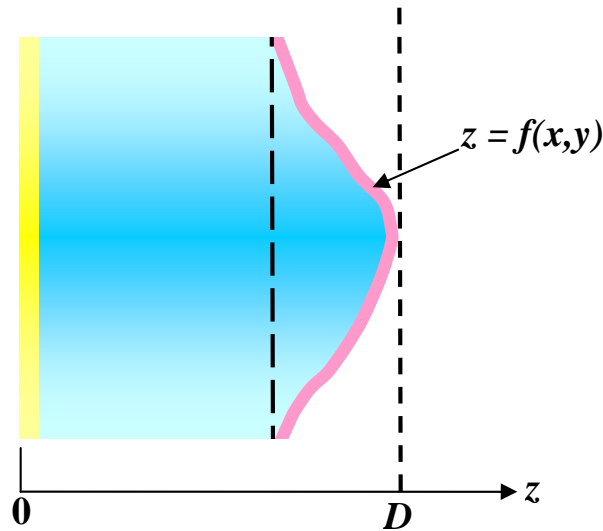
Figure 1.22: FFT based simulation methods are able to include mirrors having complicated profiles z = f(x, y) .
