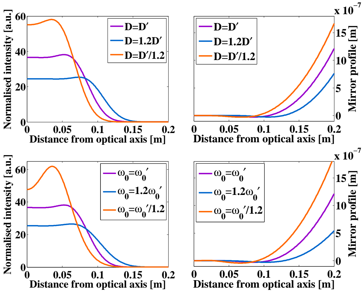
Figure 2.2: The mesa beam as a function of its parameters. In this figure primed variables denoted standard values. Upper plots: Mirror and intensity profiles (at mirror position) as a function of D for fixed \omega_0 . Lower plots: Mirror and intensity profiles (at mirror position) as a function of \omega_0 for fixed D . Studying the nominal intensity profile one understands why Willems coined the term mesa beam in reference to the landform of the same name common in the southwestern United States. Owing to their unique shape, the mesa beam mirrors have earned their own moniker. With their steep outer brim and central crown they are known as Mexican hat mirrors. 6
