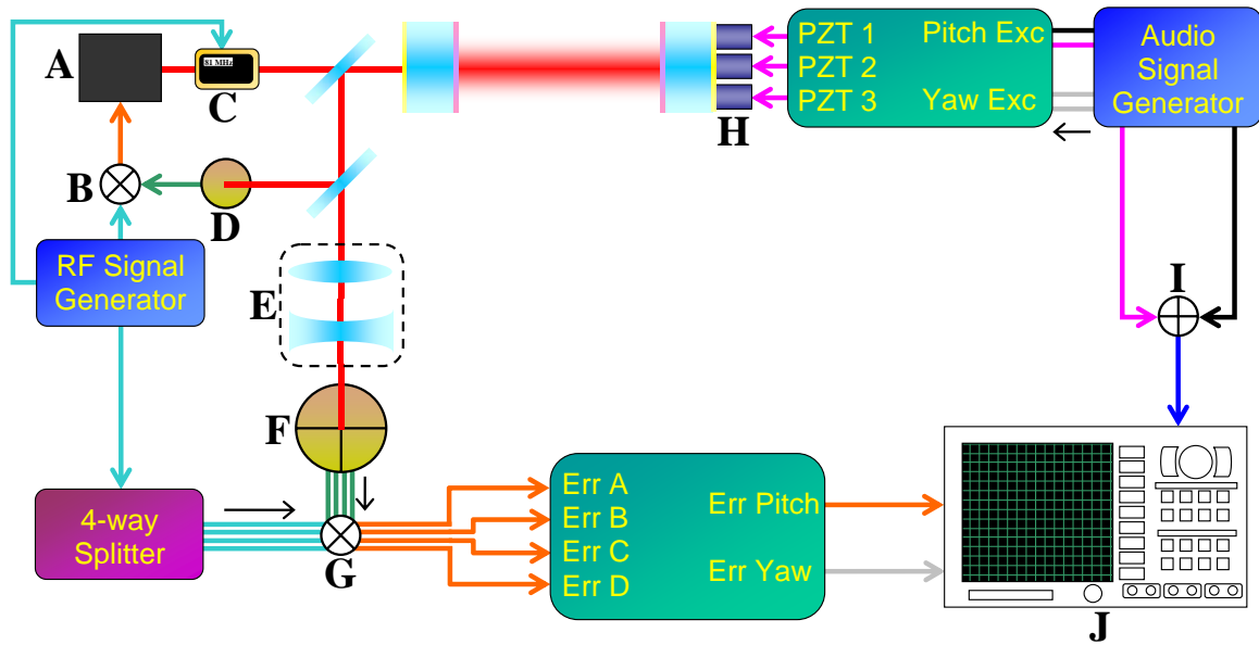
Figure 3.11: Mesa WFS experimental apparatus configured for pitch measurements. Both mirrors were excited simultaneously. Only excitations of the cavity end mirror are shown. A - Laser, B - Mixer, C - Electro-optic modulator, D - RF photodiode, E - Gouy phase telescope, F - WFS quadrant photodiode, G - Mixer, H - PZT triplet (input mirror PZTs not shown), I - Summing junction, J - Spectrum analyser.
