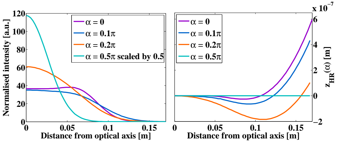
Figure 2.8: Left: Normalised intensity profiles of various hyperboloidal modes. The Gaussian \alpha = 0.5\pi mode has been reduced by a factor of two for ease of comparison. Right: The correction to the fiducial surface for each of the intensity profiles. Notice that the correction for the \alpha = 0.5\pi mode is null i.e. the mirror is spherical.
