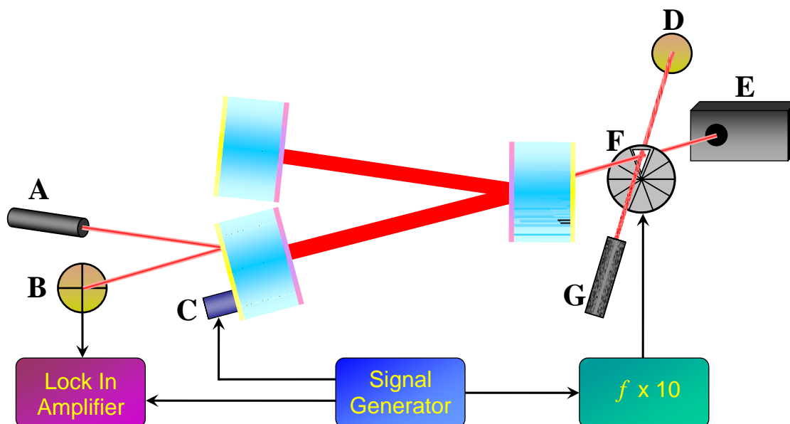
Figure 3.1: Apparatus used to measure the tilt sensitivity of the mesa beam cavity. A - He-Ne optical lever laser, B - Quadrant photodiode, C - PZT, D - DC photodiode, E - High resolution CCD camera, F - Optical chopper, G - He-Ne laser.
