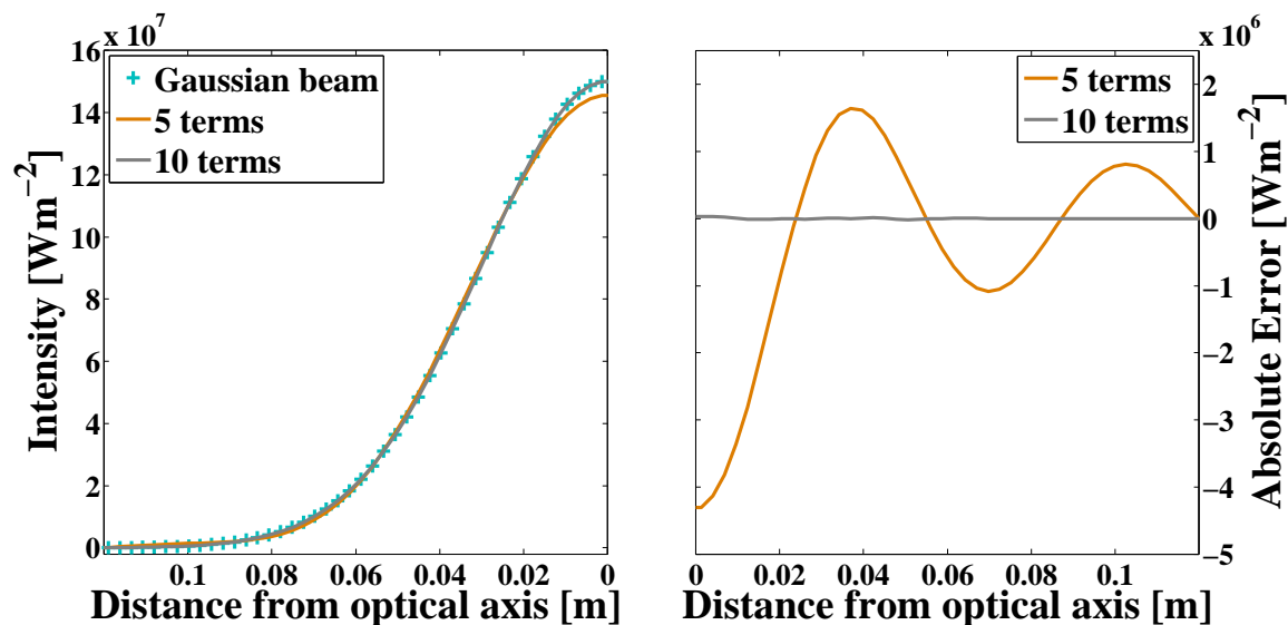
Figure 4.1: Much of the work described herein relies on Dini expansions. Here we show how efficiently the Dini expansion is able to approximate a Gaussian beam. Left: A series representation of the true intensity profile (crosses) using 5 and 10 terms. Right: Absolute error on the reconstruction.
