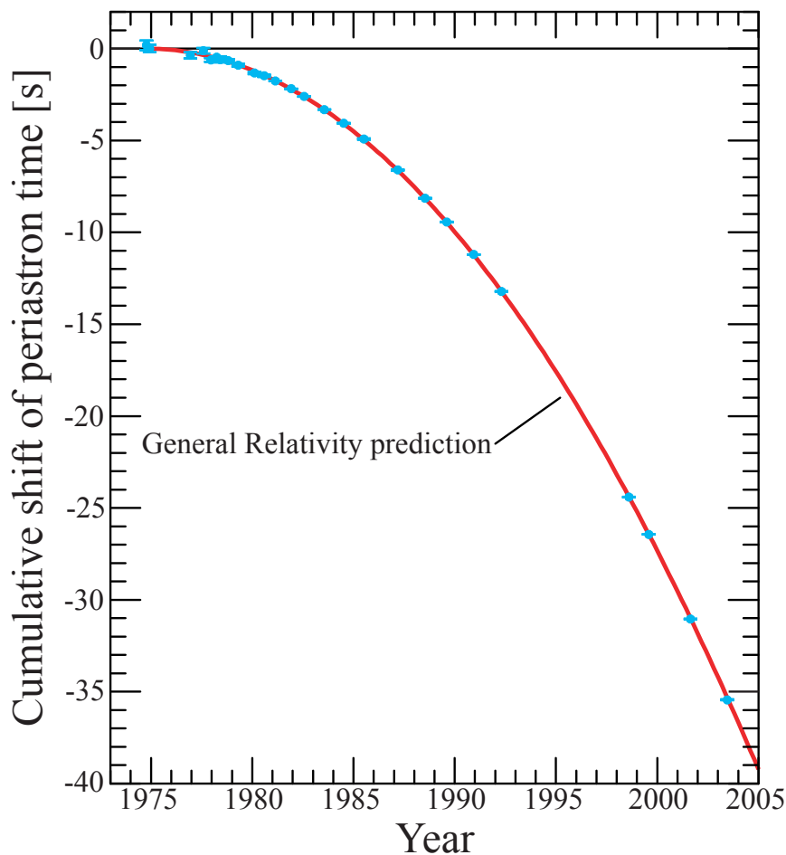
Figure 1.2: The orbit of the binary system PSR1913+16 decays exactly as if it is emitting energy in the form of gravitational waves at the level predicted by general relativity. Here the change in periastron epoch is shown as a function of time (blue) together with the general relativistic prediction (red). The orbital period of the system is \sim 0.323 days. Adapted from [15].
