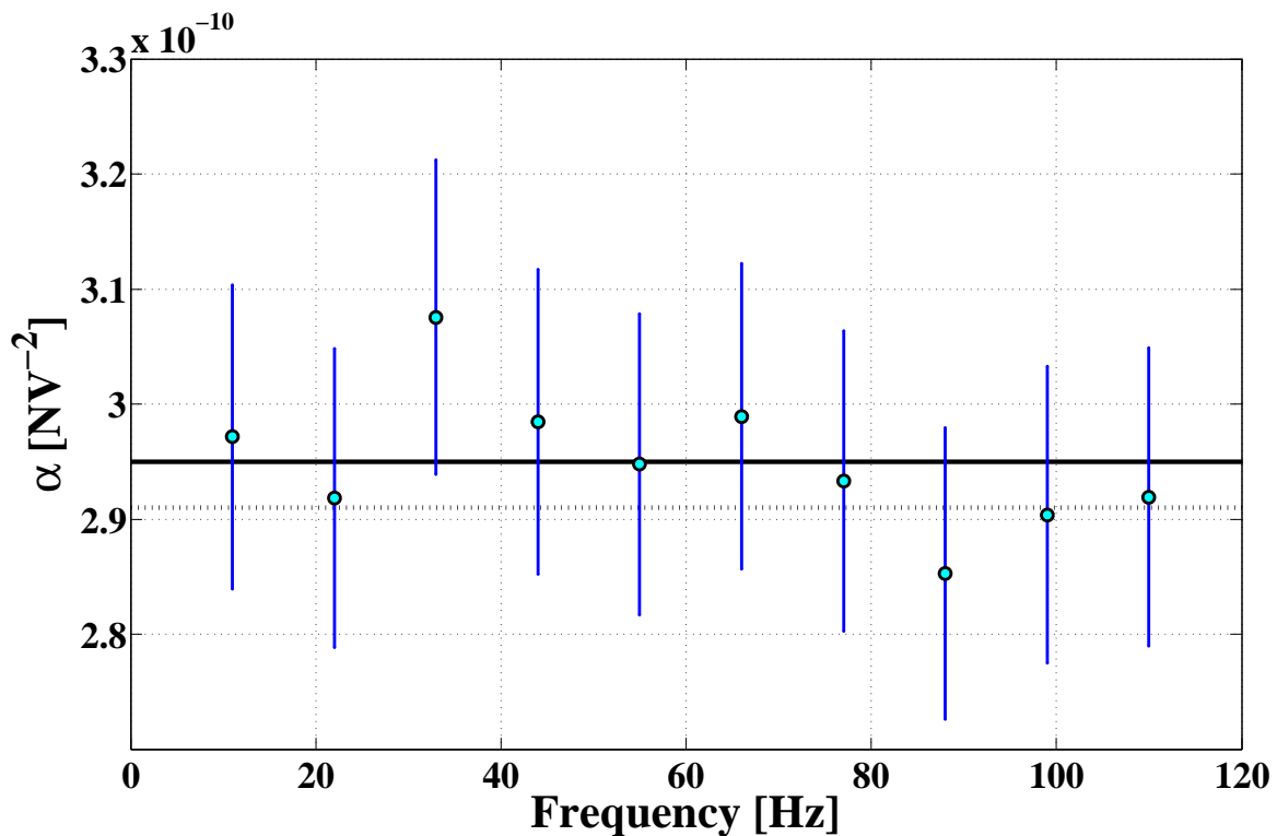
Figure 5.37: Typical ESD actuation coefficient measurement. Solid line indicates mean value of 2.95 \times 10^{-10} \text{ N/V}^2 ; dashed line shows theoretically predicted value of 2.91 \times 10^{-10} \text{ N/V}^2 .
