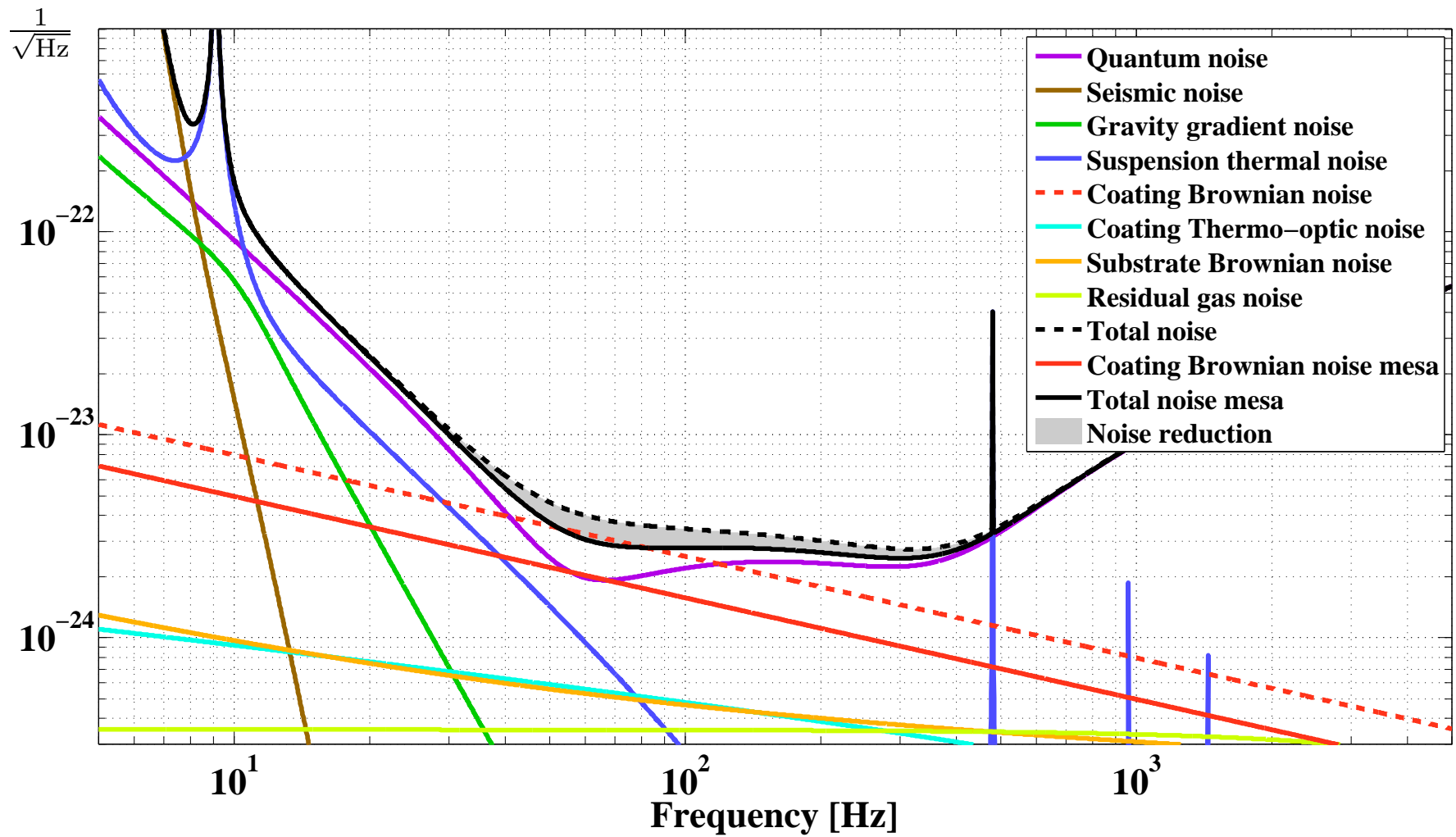
Figure 2.5: Interferometer noise curve for mesa beams with the instrument optimised for NS-NS binary inspirals.
