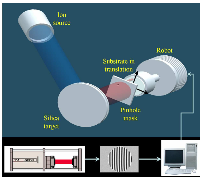
Figure 2.13: The second stage of MH mirror construction. With the substrate in translation a narrow atomic beam deposits a corrective coating to realise the fine features of the profile .
