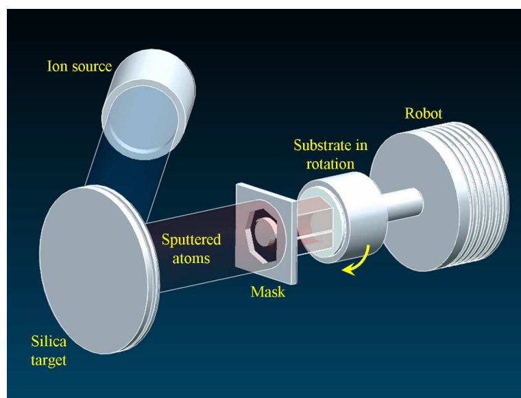
Figure 2.11: The first step in the manufacture of a MH mirror. Using a specially tapered mask (fig. 2.12) the gross features of the mirror profile are deposited with the substrate in rotation.
