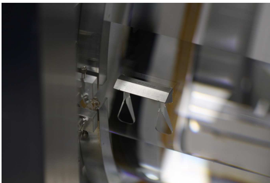
Figure 5.41: Test mass suspension wire stand off. We speculate that this item may contribute excess loss leading to low experimentally measured Q s. Below the metal standoff one can see fused silica ears to which a quasi-monolithic suspension was to be attached.
