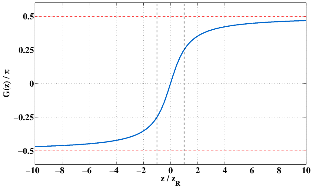
Figure 1.12: Gouy phase of a Gaussian beam upon propagation.
