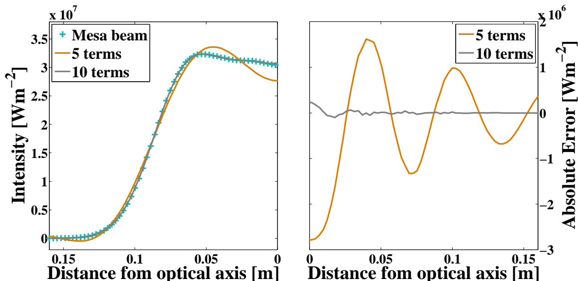
Figure 4.2: The Dini expansion is also able to accurately approximate a mesa beam. Left: A series representation of the true intensity profile (crosses) using 5 and 10 terms. Right: Absolute error on the reconstruction.
