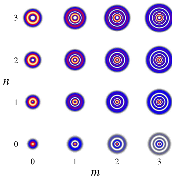
Figure 1.15: Intensity profiles of low order helical Laguerre-Gaussian modes. These modes exhibit useful radial symmetry.
