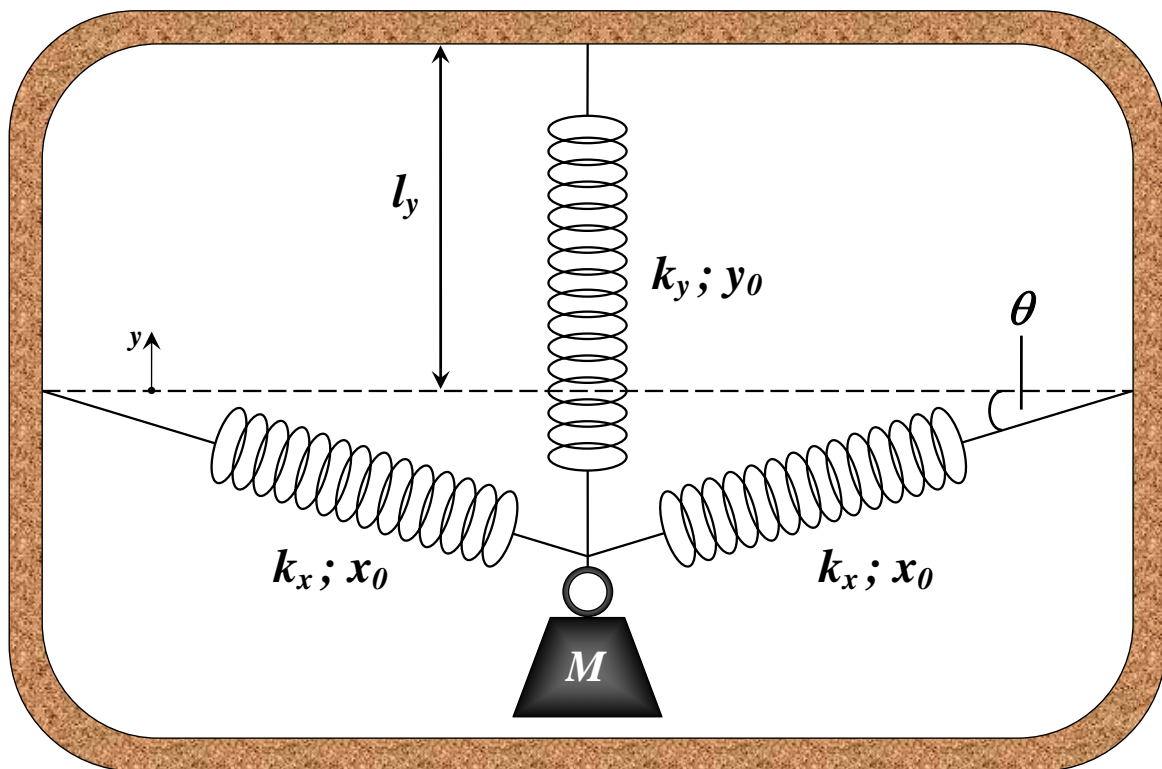
Figure 2.25: Toy model of a GAS.
