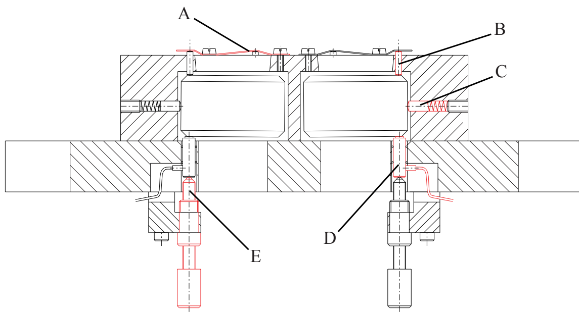
Figure 2.28: Schematic of mirror mounts and actuators. A - Annular copper beryllium spring, B - Return pin, C - Side spring and pin, D - PZT actuator, E - Micrometric screw. Each optic was endowed with three return pins, PZTs and micrometric screws. For clarity only one of each is shown.
