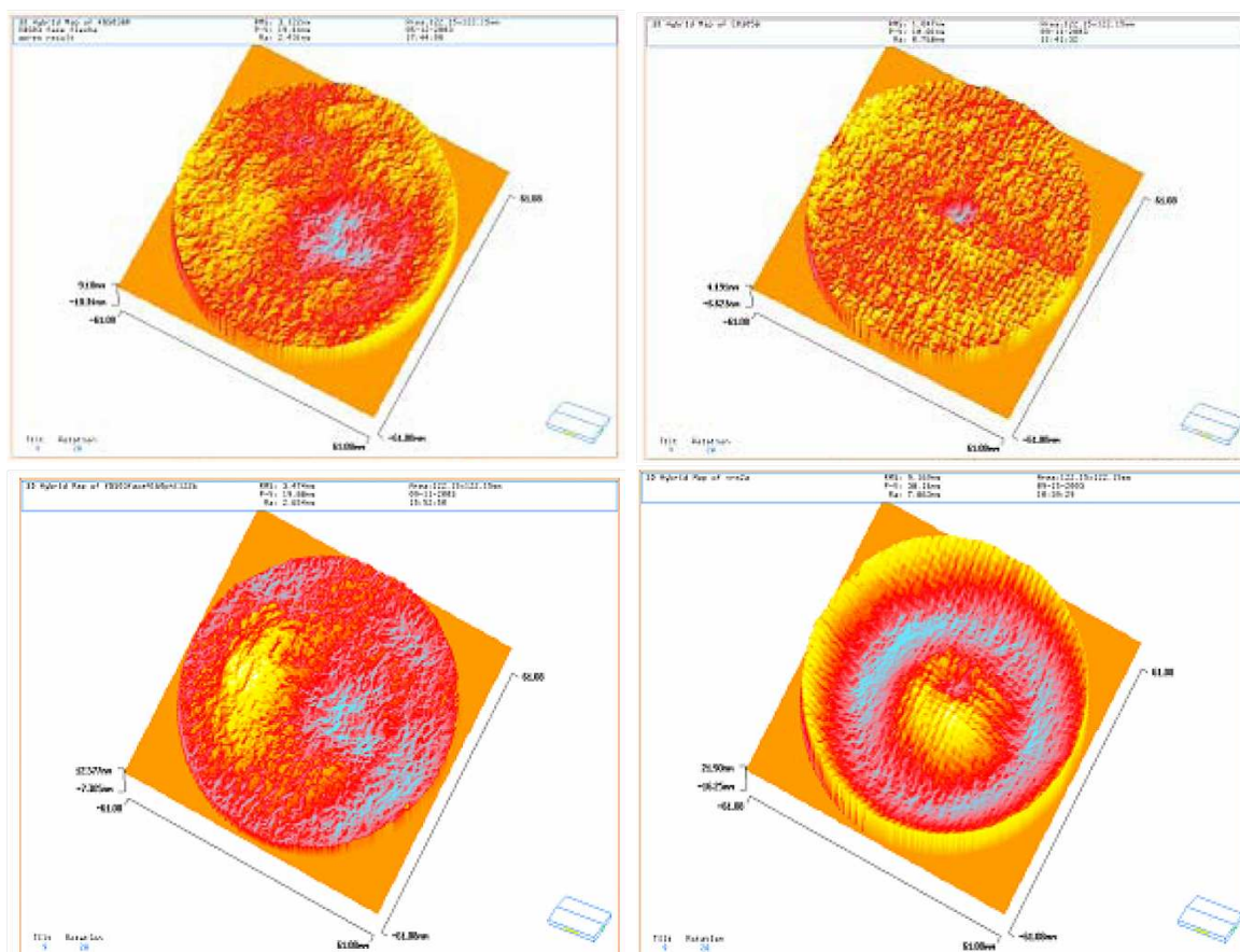
Figure 2.15: The first tests of the new deposition technique were made on opposite sides of the same substrate. Flat (upper) and MH (lower) profiles were attempted. The left hand column shows the profiles after the first deposition stage while the right shows the same surfaces after corrective coating. Both tests were successful. The small defects near the centres of both mirrors were caused by a known problem with the computer controlled translation stage. This problem was fixed before production mirrors were attempted.
