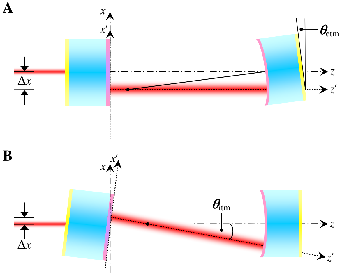
Figure 3.3: Motion of the cavity axis with mirror tilts. The unprimed system represents ideal alignment whilst the primed system follows the cavity axis as mirrors tilt. A - Tilts of the spherical mirror translate the cavity axis, B - Tilts of the plane mirror give rise to tilts and translations.
