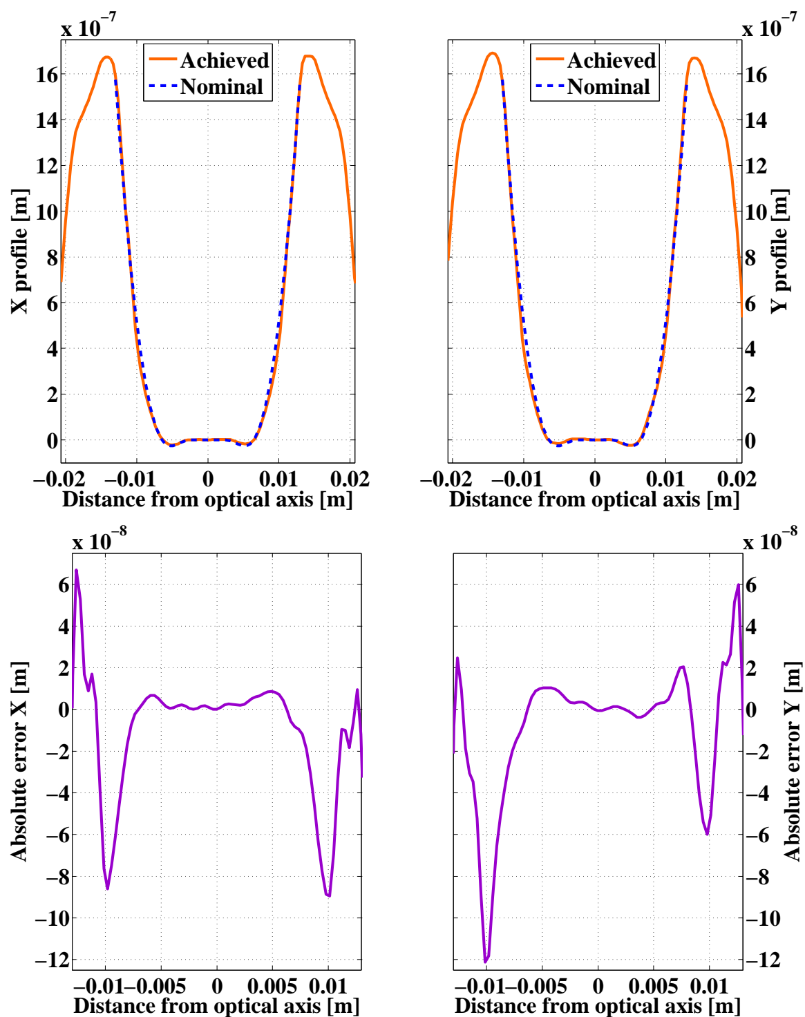
Figure 2.17: Comparison between experimental and theoretical mirrors across orthogonal profiles.
