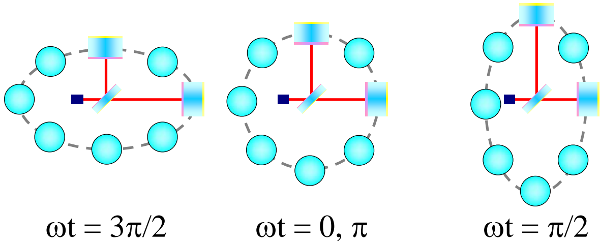
Figure 1.3: The effect of a plus-polarised gravitational wave on a Michelson interferometer with suspended mirrors.
