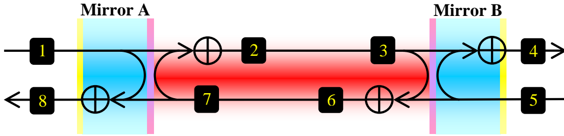
Figure 5.2: Node diagram of a Fabry-Perot cavity used to construct matrix of transfer coefficients.
