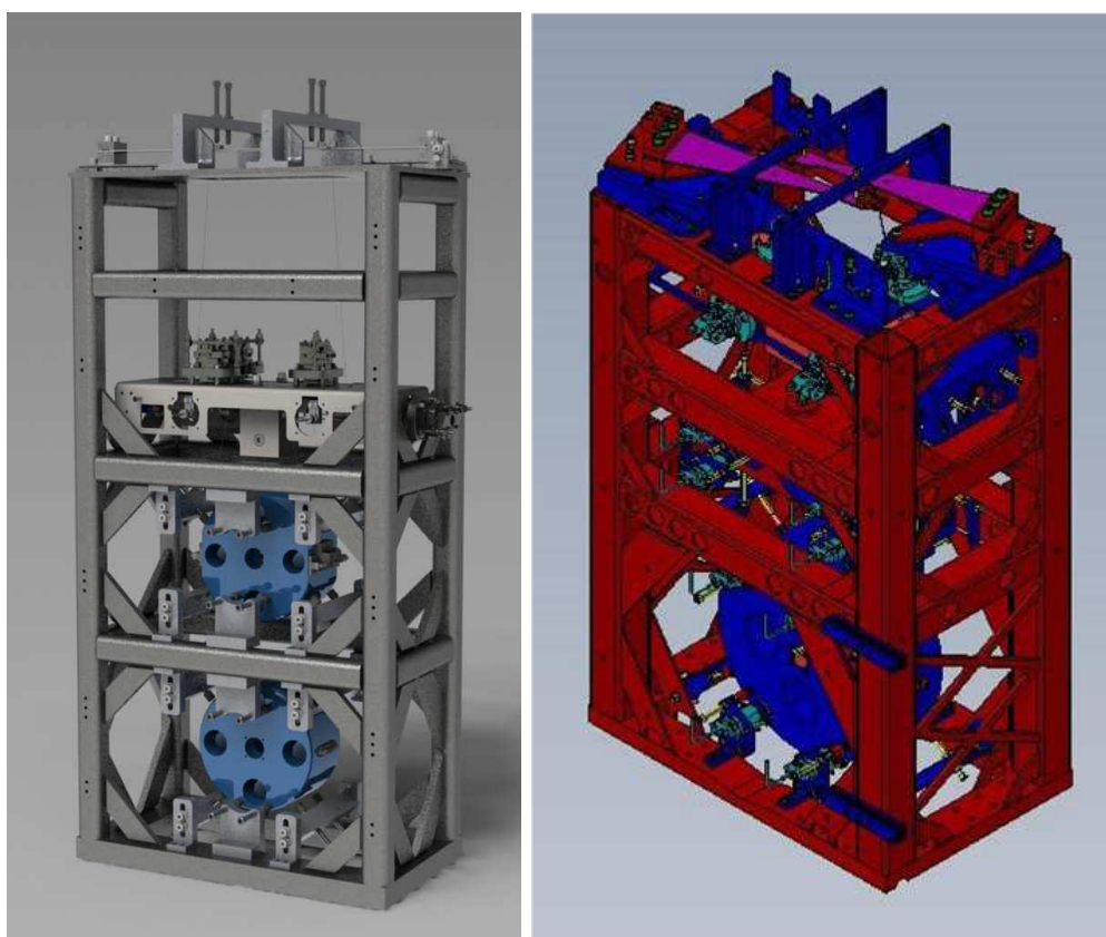
Figure 5.27: Left: HAM small triple suspension designed for 150 mm diameter optics. This design is appropriate for the input mode cleaner mirrors and the small recycling cavity optics. Right: HAM large triple suspension for 265 mm diameter optics. This design shall be used for the large recycling cavity mirrors. There exists a third triple suspension (not shown) for beam splitters and folding mirrors.
