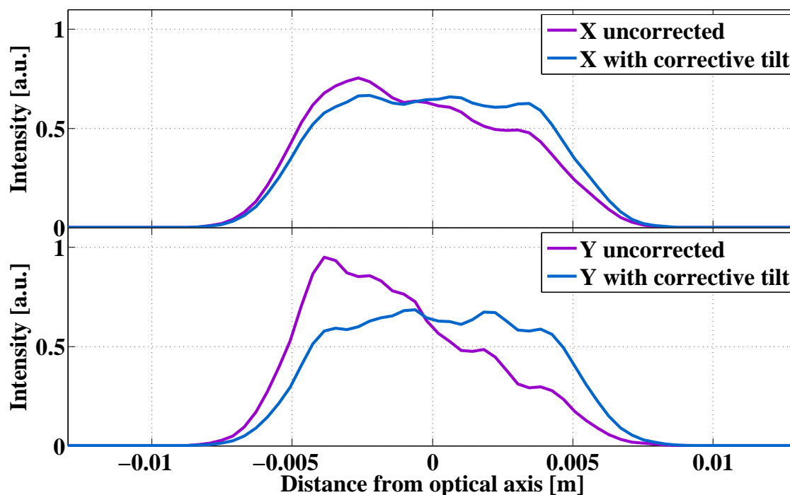
Figure 2.19: Applying a corrective tilt of order 0.9 \mu\text{rad} mitigated manufacturing errors which left the central area of the MH optic tilted with respect to the mirror's fiducial plane (see fig. 2.18).
