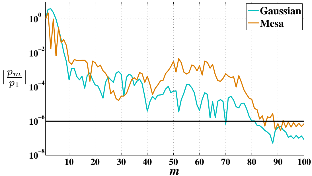
Figure 4.3: Dini expansions are able to reconstruct the incident optical intensity profile with a minimum of terms. In our analysis we incorporate all terms with expansion coefficients greater than 10^{-6} times the first term p_1 . For nominal mode shapes this corresponds to more than 80 terms.
