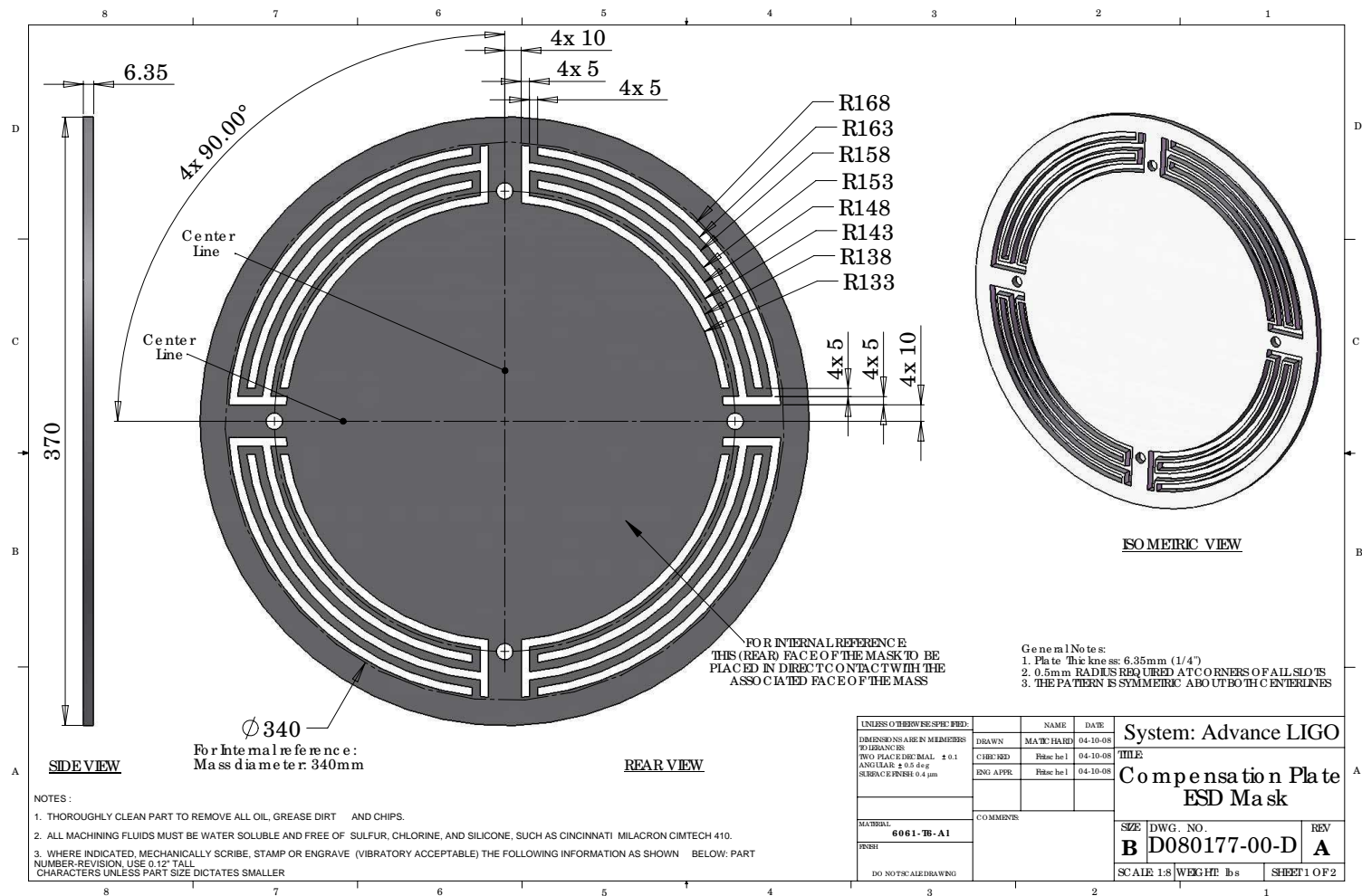
Figure B.1: Technical drawing of mask used in manufacture of LASTI prototype ESD (1 of 2). We assume perfect manufacturing and use the dimensions given in our model.
