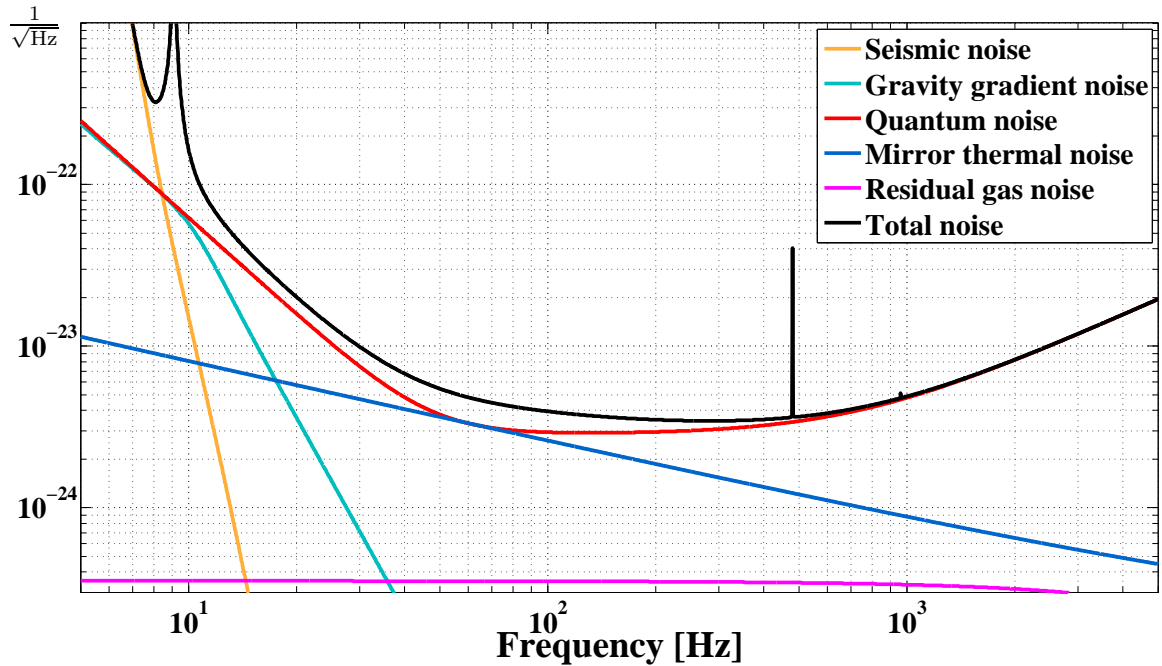
Figure 1.9: Noise from selected sources described in terms of equivalent strain noise. Quantum noise encompasses both radiation pressure noise and shot noise.
