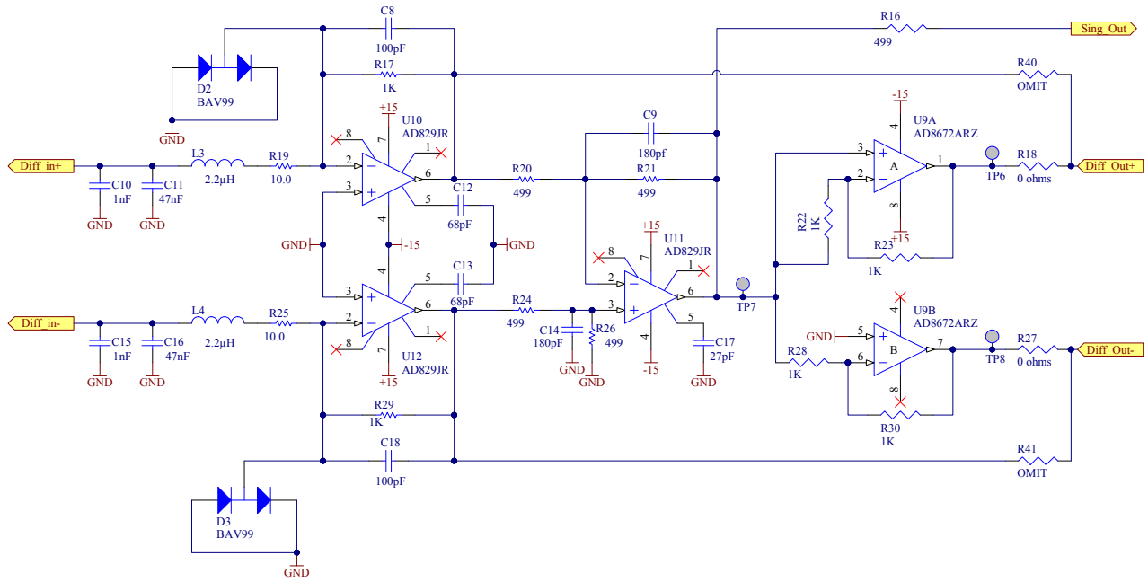
Figure 3 IF Output Amplifier
