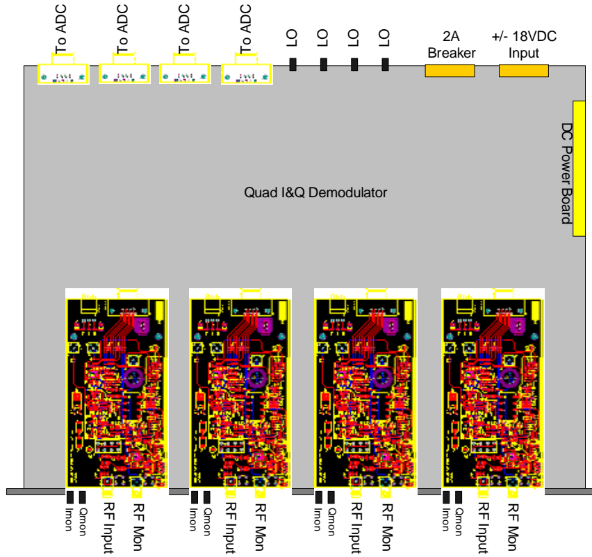
Figure 6 Demodulator Chassis
