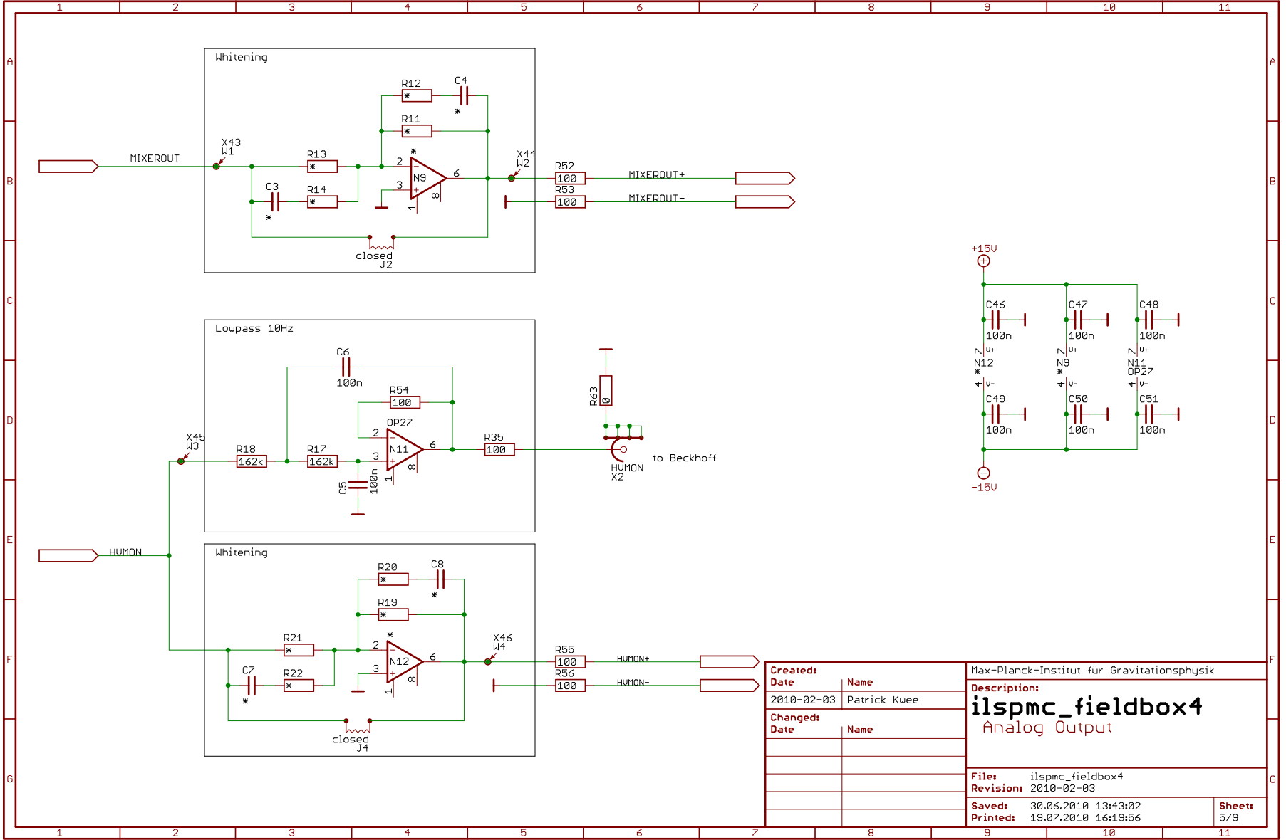
Figure 5: Project schematics (sheet 5)
