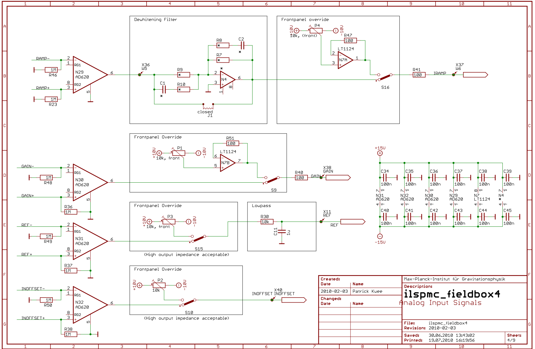
Figure 4: Project schematics (sheet 4)
