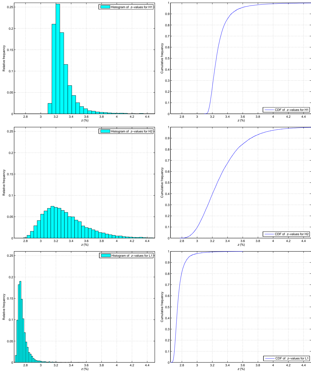
Figure 1. Frequency histograms and empirical cumulative distributions for z (expressed as a percentage).
