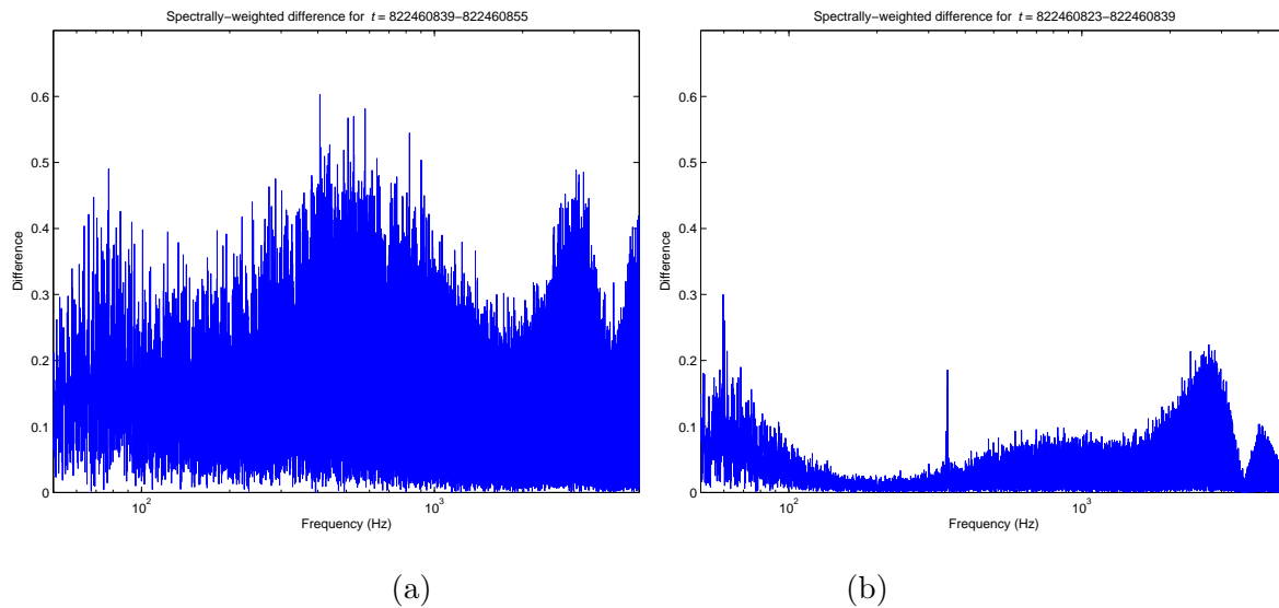
Figure 2. Pointwise difference \frac{2|\tilde{h}^e(f) - \tilde{h}(f)|}{\sqrt{S(f)}} in H1 data for (a) the interval giving the largest z and (b) the preceding interval.
