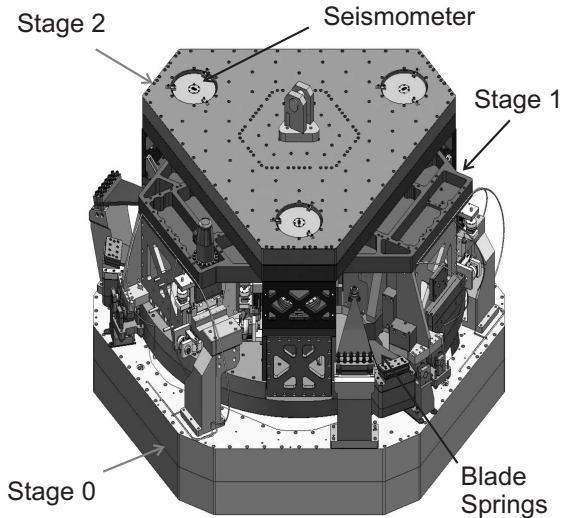
Figure 4. Internal stages of the large chamber seismic isolation subsystem. The hydraulic actuators support tubes outside the vacuum which cross into the vacuum tanks and support Stage 0 of the internal isolation. Stage 1 is supported from Stage 0 by the maraging steel blade springs, as is Stage 2 from Stage 1. A vertical seismometer in Stage 2 is also shown.
