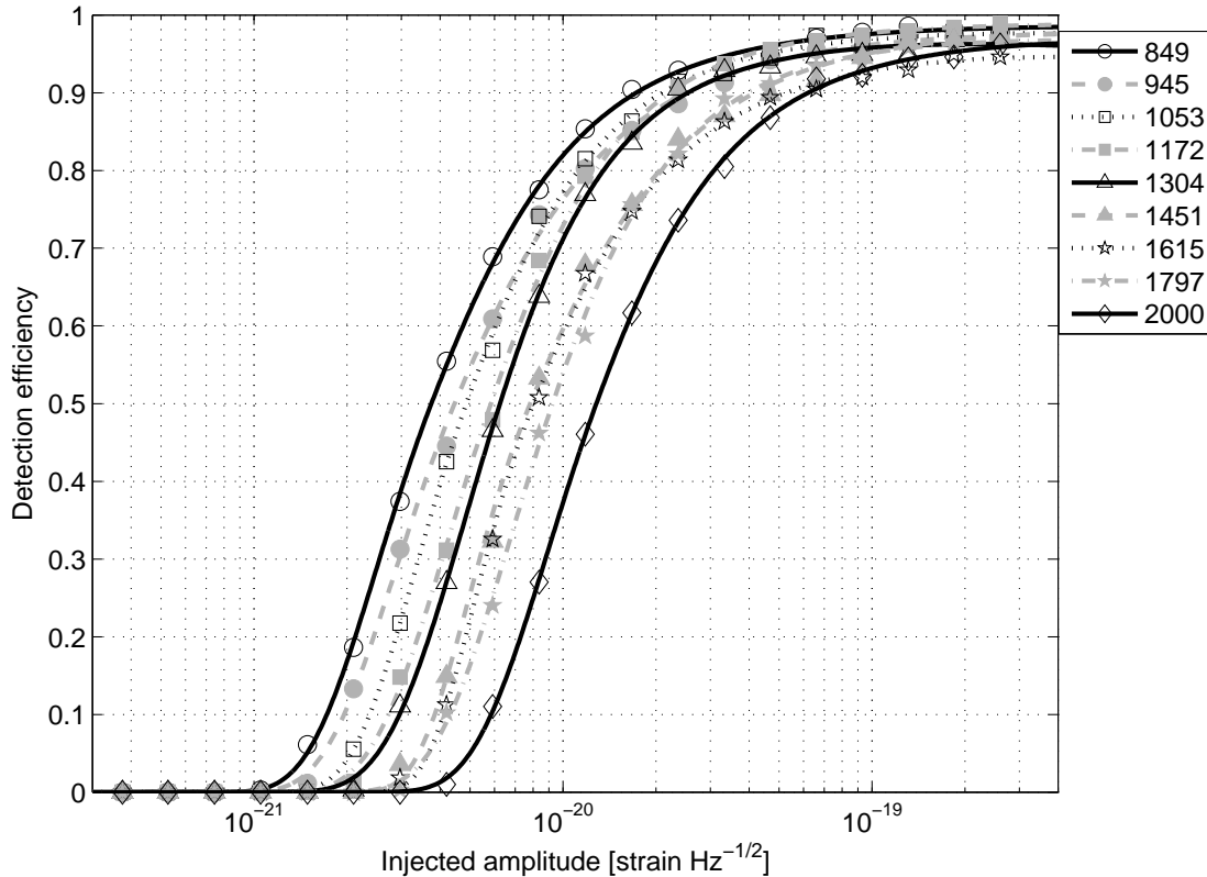
Figure 7. Detection efficiency of the coherent Waveburst pipeline for various sine-Gaussian simulated gravitational-wave bursts, as a function of the signal amplitude (defined by Eq. 15). The legend indicates the central frequency (Hz) of the injected signal and the h_{\text{rss}}^{50\%} ( \text{Hz}^{-1/2} ) sensitivity of the pipeline.
