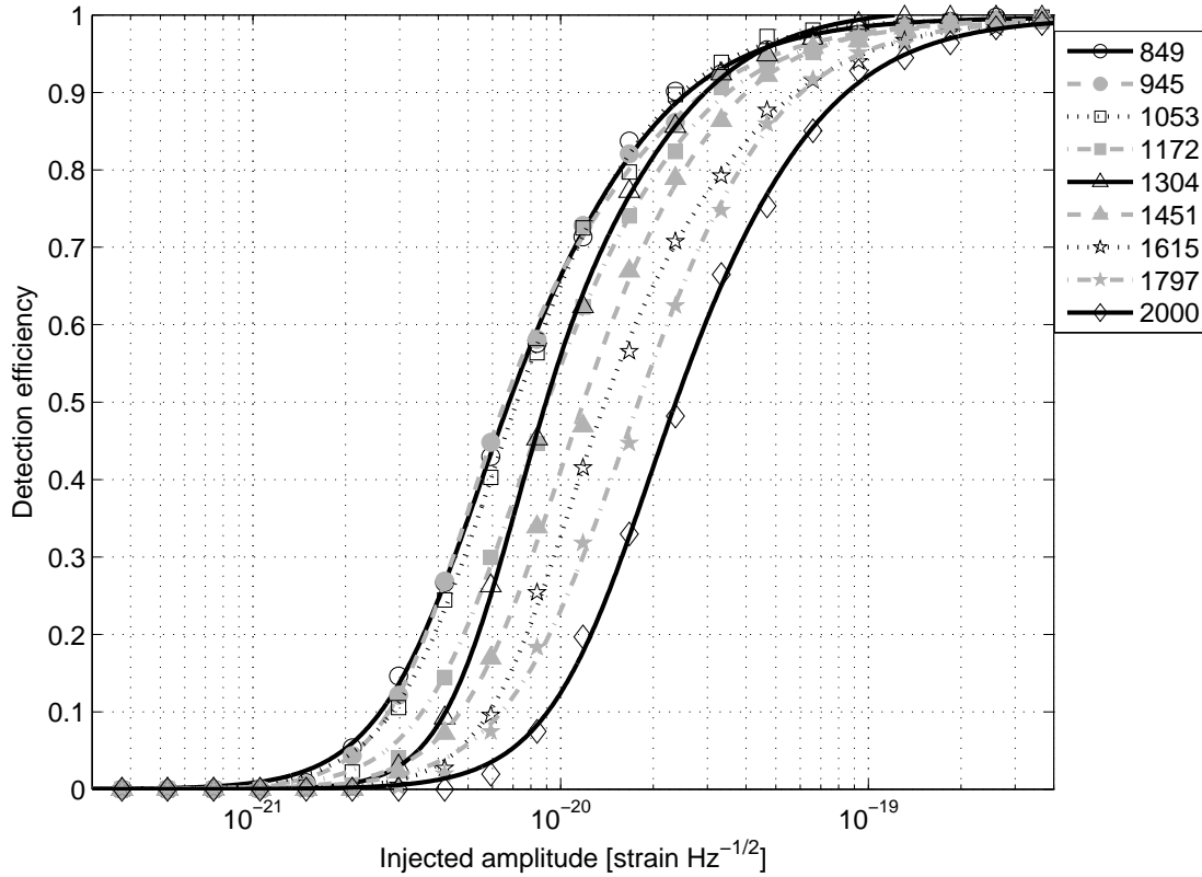
Figure 5. Detection efficiency for WBCP pipeline for sine-Gaussians with different central frequencies.
