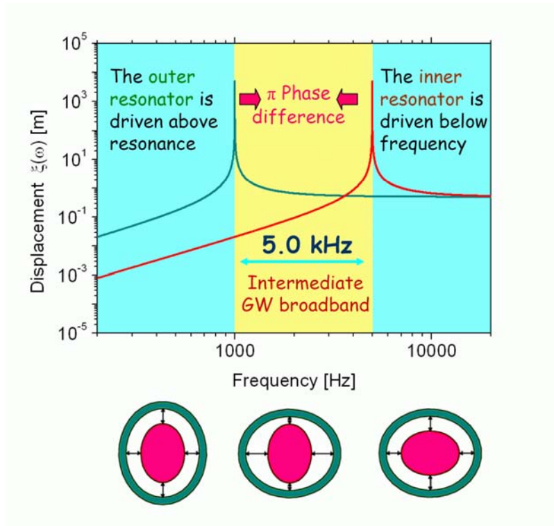
Figure 11. Illustration showing the DUAL detector operation. The two nested oscillators in the lower part of the figure illustrate how it operates: above and below both resonances the two oscillators respond to a gravitational wave with the same phase, but between the two resonances they respond out of phase. Transducers in the gap will sense the differential motion. (Figure courtesy of the DUAL Collaboration.)
