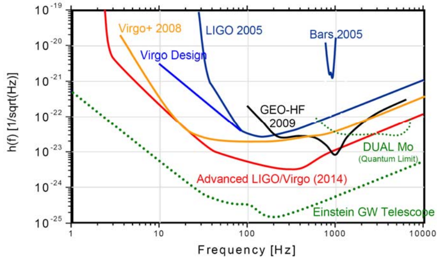
Figure 10. Possible noise level for the Einstein Gravitational-Wave Telescope compared with the other current and planned detectors. (Figure courtesy of the ET Collaboration.)
