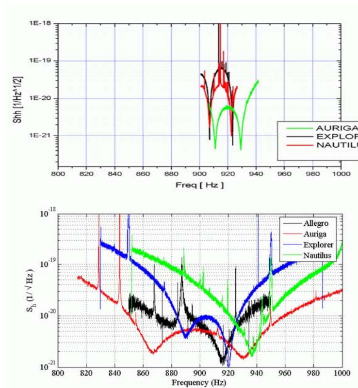
Figure 1. Strain sensitivity (noise level) versus frequency for the four current IGEC bar detectors. The top plot shows the sensitivities in the IGEC-1 run (1997-2000), while the bottom one shows the sensitivities as improved for the IGEC-2 run (2005-on). The improved bandwidth increases the sensitivity for broadband sources approximately proportion to the square root of bandwidth. (Figure courtesy of the IGEC-2 Collaboration [9] and reprinted with permission from Astone P et al , Phys Rev. D 76 102001 (2007). Copyright 2007 by the American Physical Society.)
