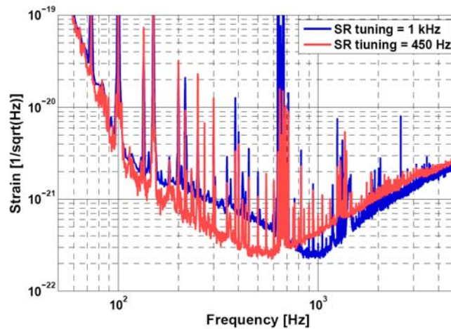
Figure 5. Strain sensitivity (noise level) versus frequency for the GEO600 detector, showing how the sensitivity can be tailored by tuning the position of the signal-recycling mirror. (Figure courtesy of the GEO Collaboration and the Institute of Physics [14].)
