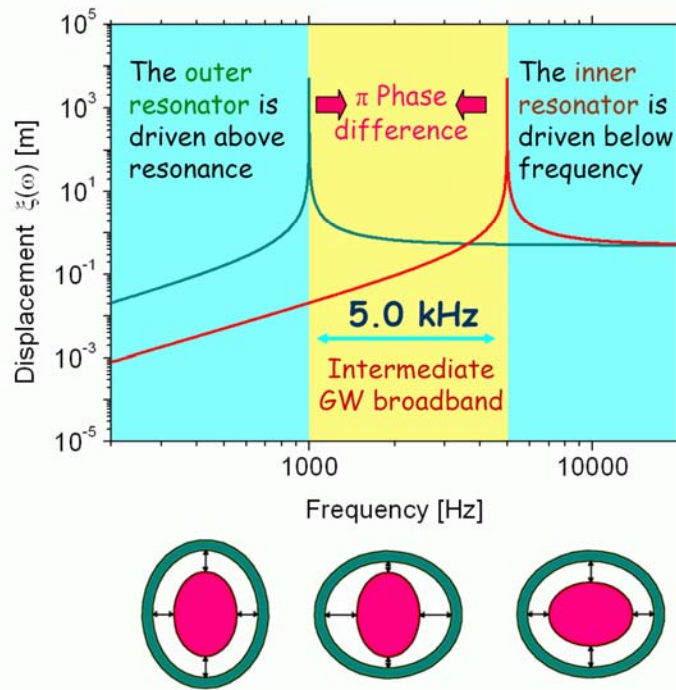
Figure 11. Illustration showing the DUAL detector operation. The two nested oscillators in the lower part of the figure illustrate how it operates: above and below both resonances the two oscillators respond to a gravitational wave with the same phase, but between the two resonances they respond out of phase. Transducers in the gap will sense the differential motion. (Figure courtesy of the DUAL Collaboration.)
