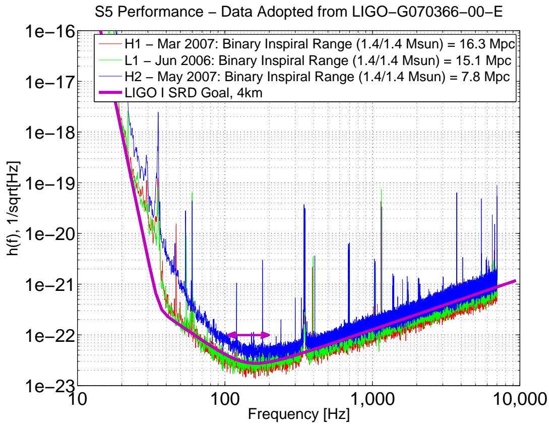
Figure 2. Performance of the Hanford 4km instrument (red), Livingston 4km instrument (green) and Hanford 2km instrument (blue) in S5, plotted as linear spectral density of the strain noise. The arrow represents the design sensitivity, and “LIGO I SRD” is from the initial design parameters for 4km instruments to realize the design sensitivity.
