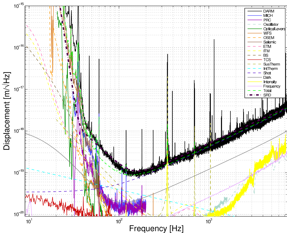
Figure 3. Projection of various noise sources coupling to the displacement sensitivity of the H1 detector. DARM: Displacement noise of the H1 instrument. MICH and PRC: Noise of the auxiliary servo controlling the Michelson part and the power recycling cavity part of the interferometer. Oscillator: Local oscillator noise. OpticalLevers and OSEM: Noise of servos locally damping the angle and position of the mirrors. WFS: Noise of the wave front sensors controlling the angle of the mirrors. Seismic: Noise caused by seismic excitation. ETM, ITM and BS: Actuator noise of End Test Masses, Input Test Masses and Beam Splitter. TCS: Noise coming from the thermal compensation system. SusTherm and IntTherm: Thermally excited motion of the wires suspending the mirrors and the internal resonant modes of the mirrors. Shot: Shot noise. Dark: Noise of the main detection electronics chain. Intensity and Frequency: Intensity and frequency noise of the laser. Total: Root sum square of all of the noise contributions. SRD: See Fig. 2.
