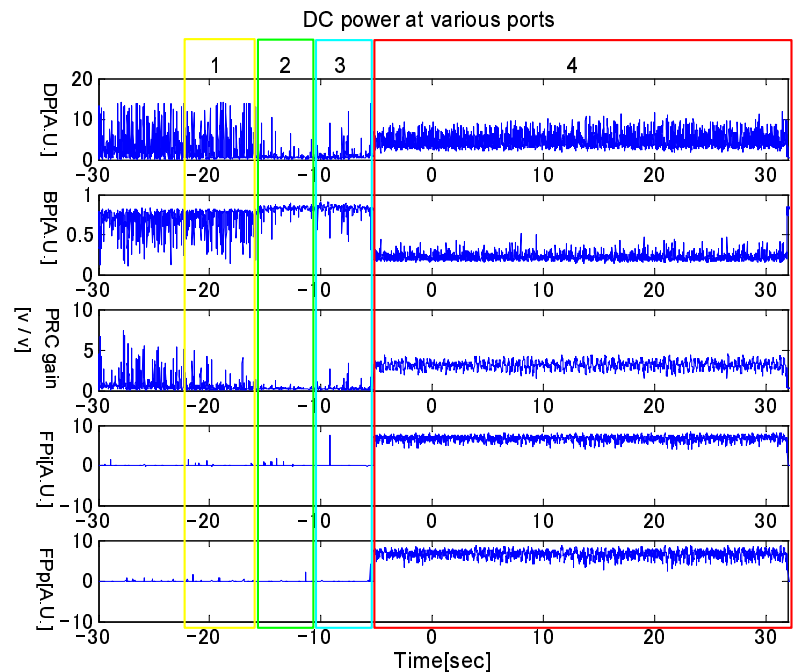
Figure 6. DC power at various ports.
