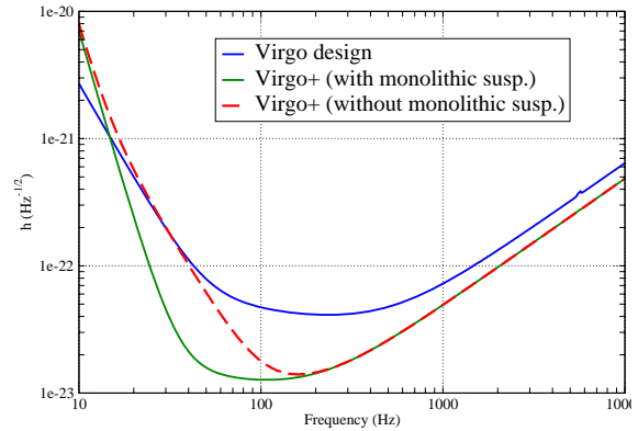
Figure 3. Virgo+ sensitivity.
