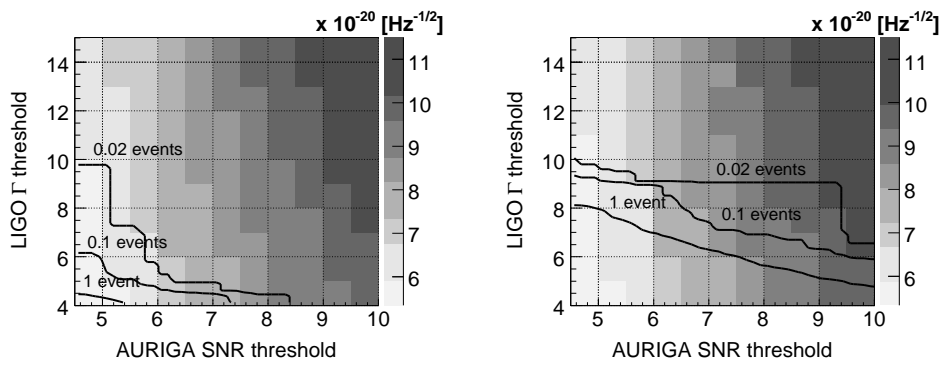
Figure 4. Grayscale plot: efficiency to sine-Gaussians waveforms in terms of h_{rss} 50%. Left: 4-fold; right: 3-fold observations. The contour lines indicate the number of accidental coincidences expected in the on-source data set.
