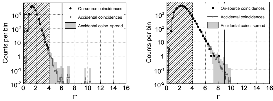
Figure 8. Comparison of \Gamma distributions for four-fold (left) and three-fold coincidences (right). The black dots correspond to on-source coincidences. The stair-step curve with gray dots is the mean accidental background, estimated from off-source coincidences, with its 1\sigma RMS spread (shaded gray area) and the error on the mean (thin error bars). The on-source and off-source distributions are in good agreement, within the statistical uncertainty. The solid vertical lines correspond to the analysis thresholds ( \Gamma = 6 and \Gamma = 9 , respectively). The analysis was tuned only on events with \Gamma \geq 4 (dotted vertical lines).
