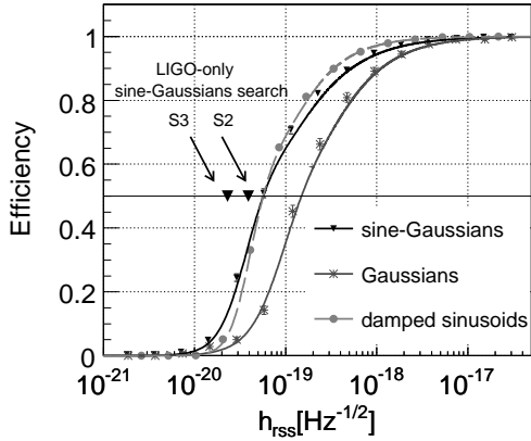
Figure 6. Average efficiency of detection (4-fold+3-fold) versus h_{rss} for the considered waveforms: sine-Gaussians at f_0 = 900 Hz and \tau = 2.2 ms, Gaussians with \tau = 0.2 ms, and damped sinusoids with f_0 = 930 Hz and damping time \tau = 6 ms. All sources have been modelled as uniformly distributed in the sky and with random polarizations (see section 2.2). The triangles mark the h_{rss} 50% for sine-Gaussians achieved in the LIGO-only S2 and S3 searches.
