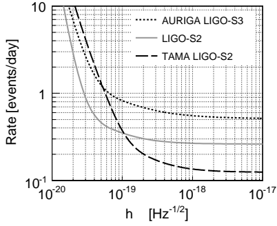
Figure 7. Upper limits at 90% C.L. on the gravitational wave rate versus h_{rss} for sine-Gaussian waveforms in different network analyses: AURIGA-LIGO S3 (dotted line), LIGO-only S2 (solid line) and TAMA-LIGO S2 (dashed line). The sine-Gaussians have central frequency 900 Hz (for AURIGA-LIGO S3) and 850 Hz (for LIGO-only S2 and TAMA-LIGO S2). In all cases, Q = 8.9 . All sources have been modelled as uniformly distributed in the sky and with random polarizations (see section 2.2)
