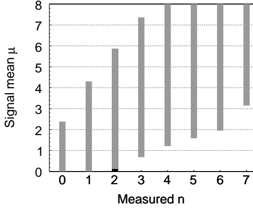
Figure 5. Confidence belt based on the Feldman and Cousins procedure, with 90% C.L., unknown Poisson signal mean \mu and a Poisson background with b = 0.24 \pm 3\sigma . The standard Feldman and Cousins construction (solid lines) is modified by fixing the maximum false alarm probability to 1%: the lower bound is fixed to 0 for 2 measured events.
