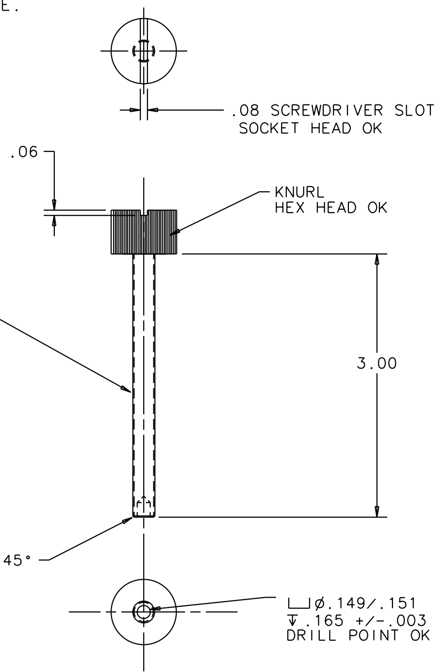
SCREW DETAIL ITEM 1
