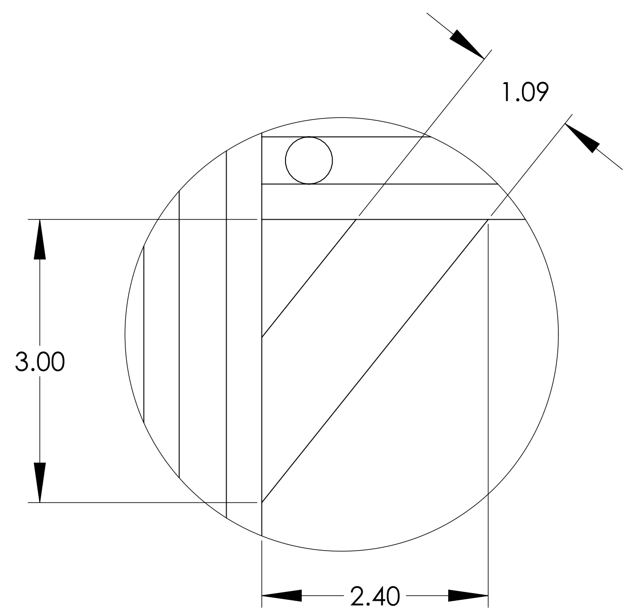
DETAIL B SCALE 1 : 1 6 PLACES
