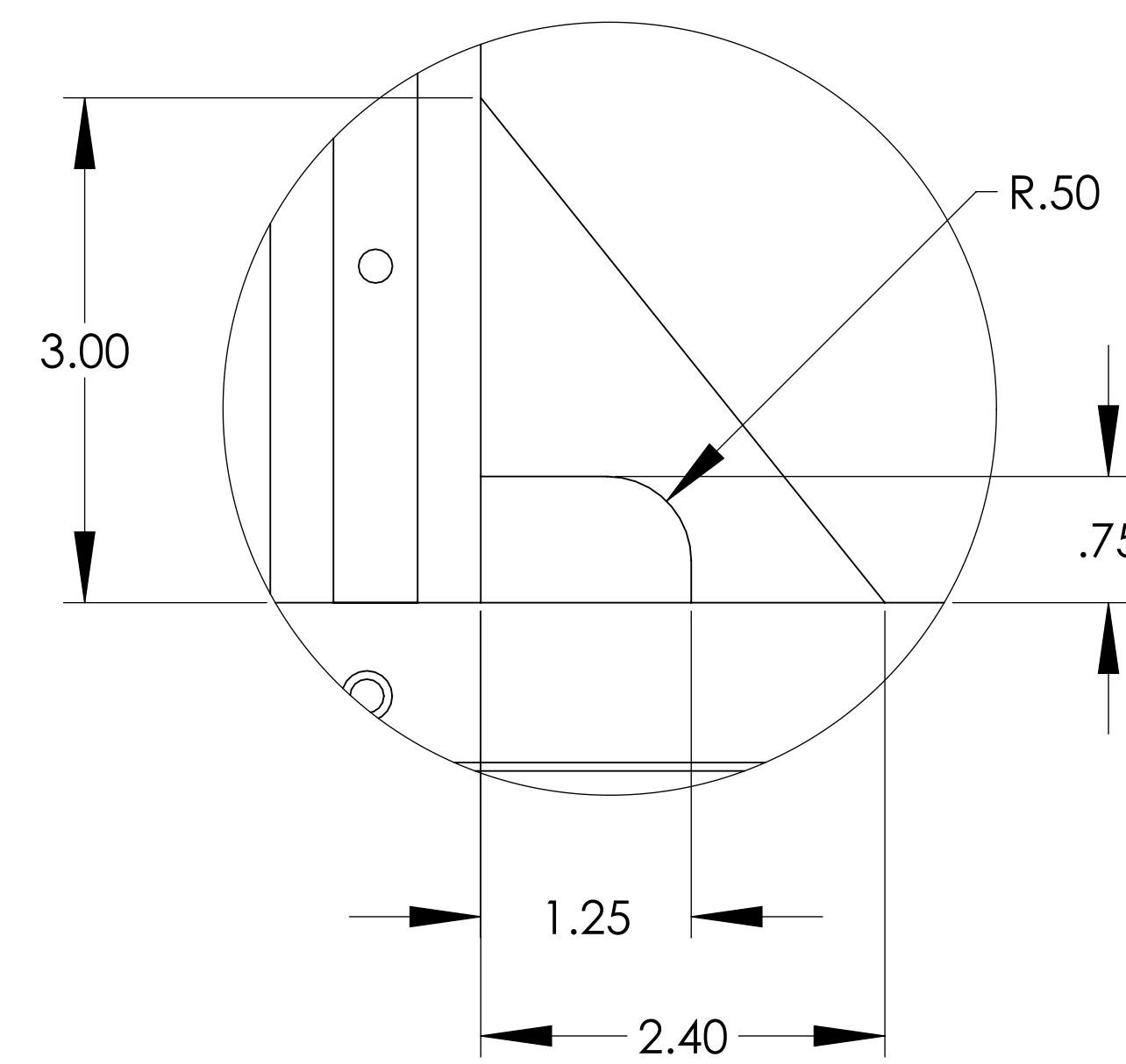
DETAIL C SCALE 1 : 1 2 PLACES
