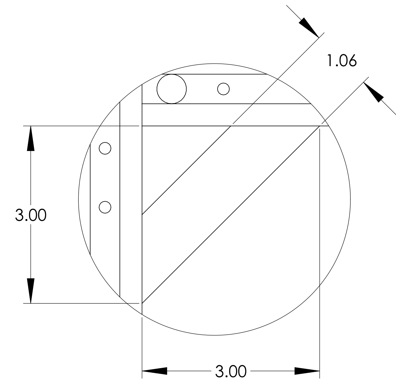
DETAIL A SCALE 1 : 1 2 PLACES
