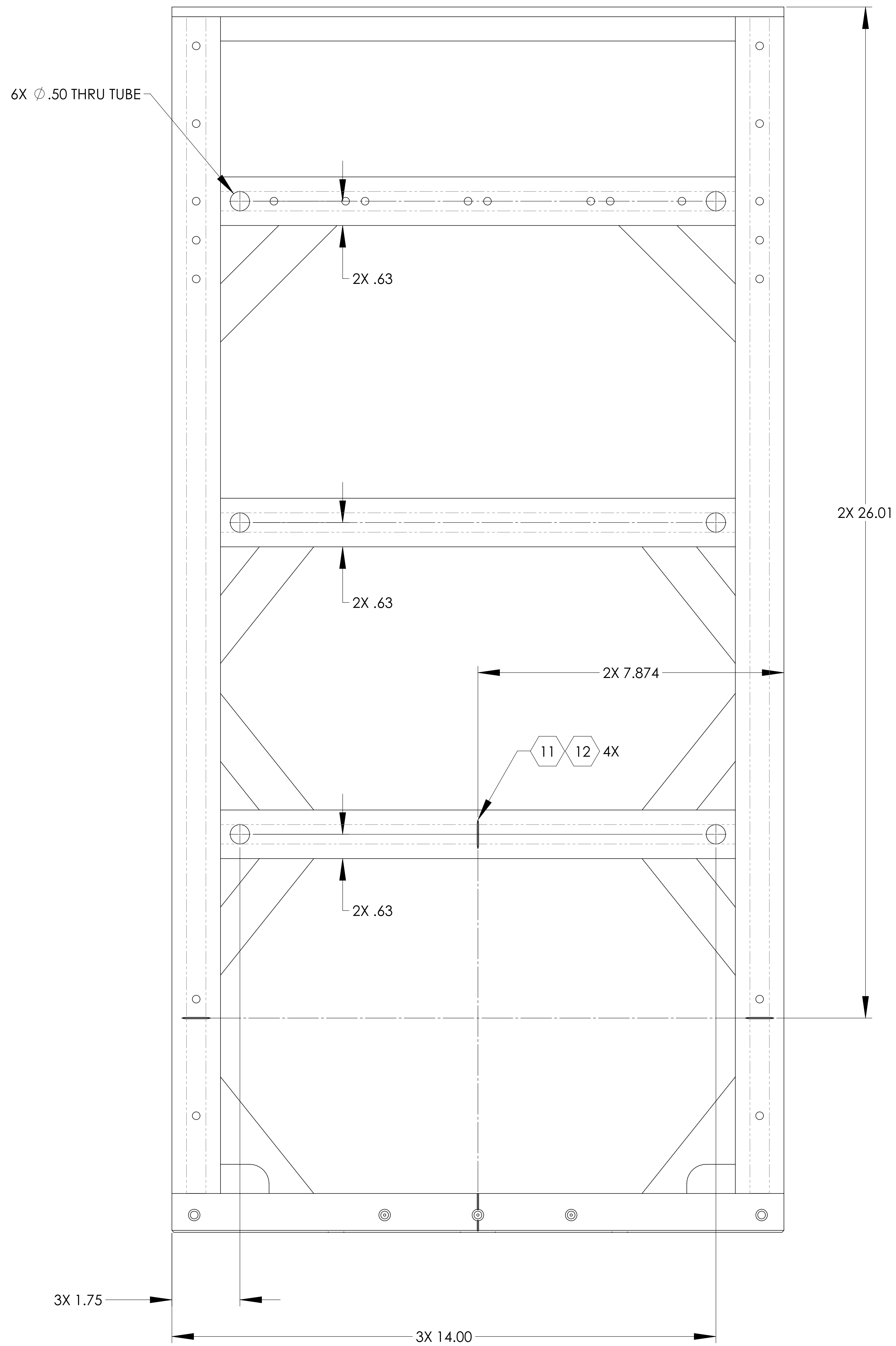
FRONT AND BACK SIDES
