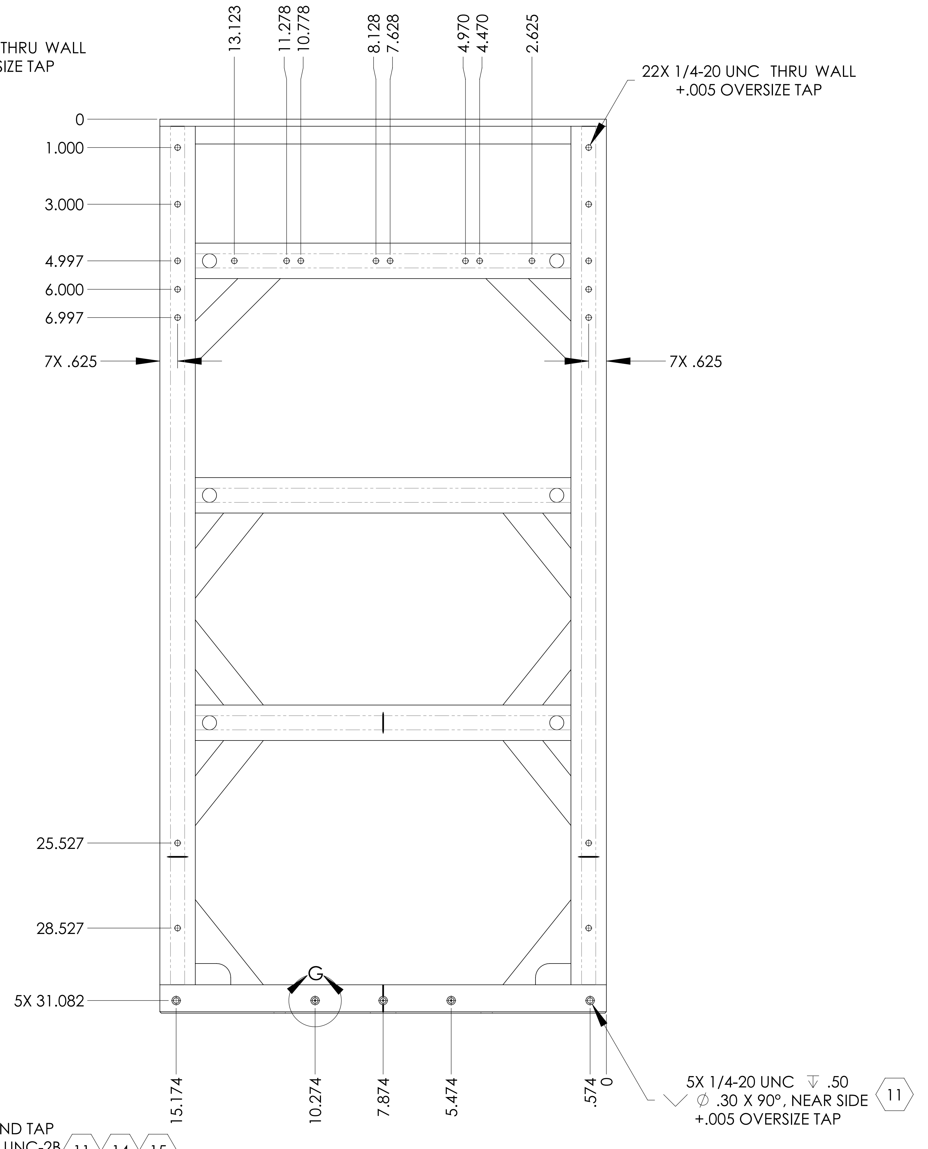
FRONT AND BACK SIDES
