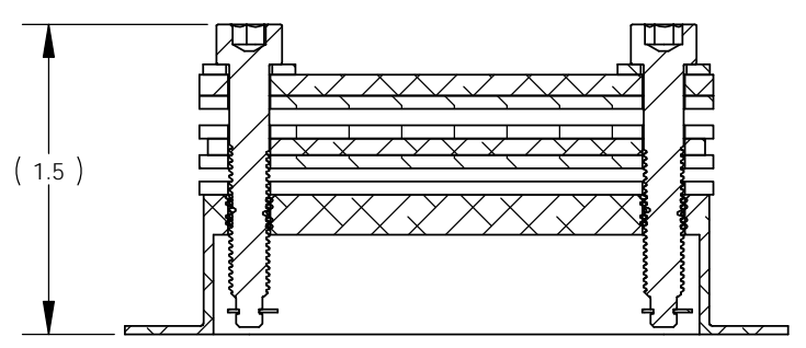
SECTION A-A (FULLY COMPRESSED)
