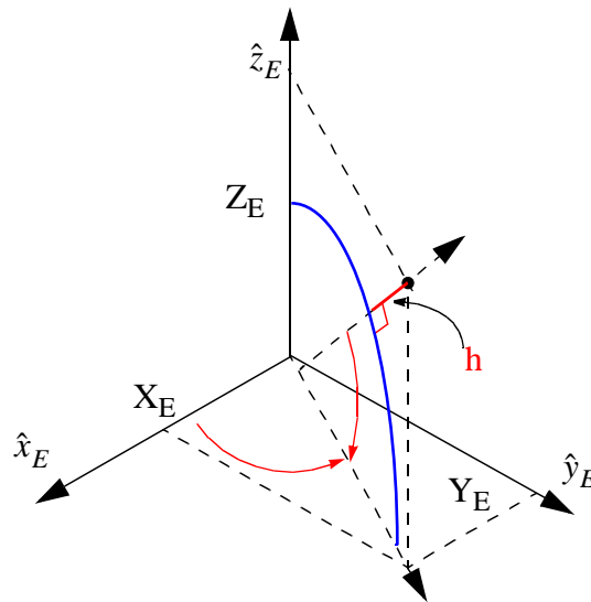
Figure 1: Geodetic and Earth-Fixed Coordinates
