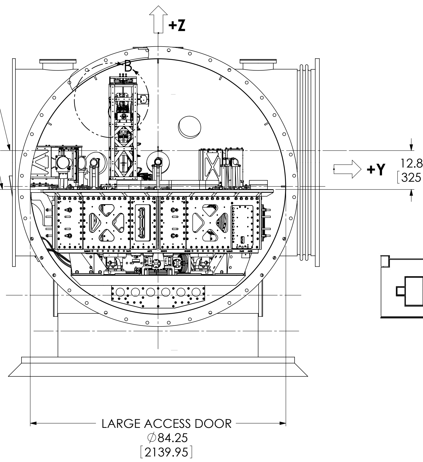
RIGHT VIEW
