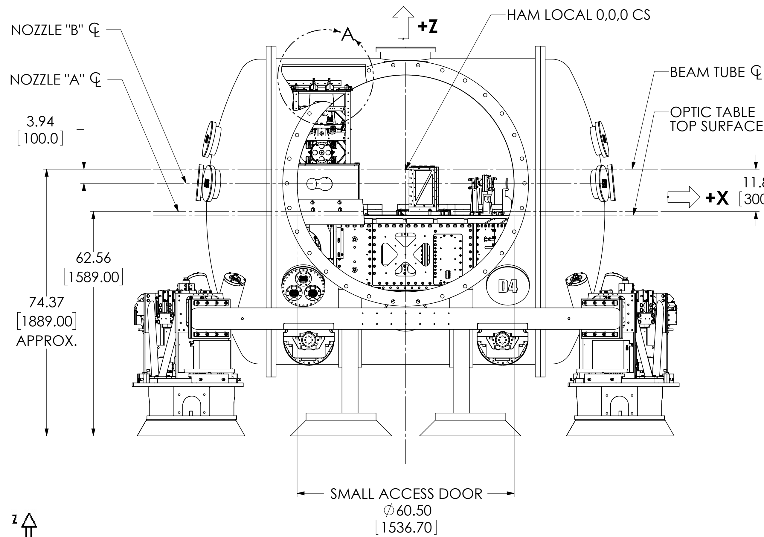
FRONT VIEW
