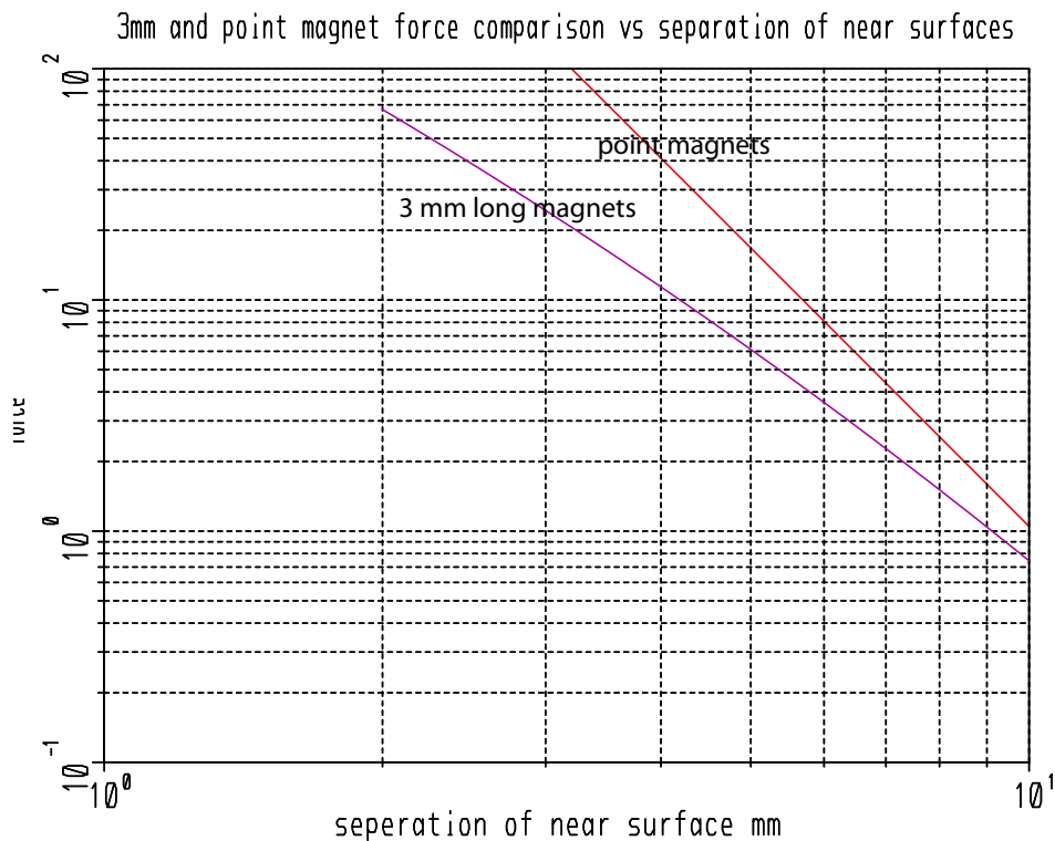
Figure 1 Scaling of the force with separation between 3mm long magnets and the scaling of point magnets.
