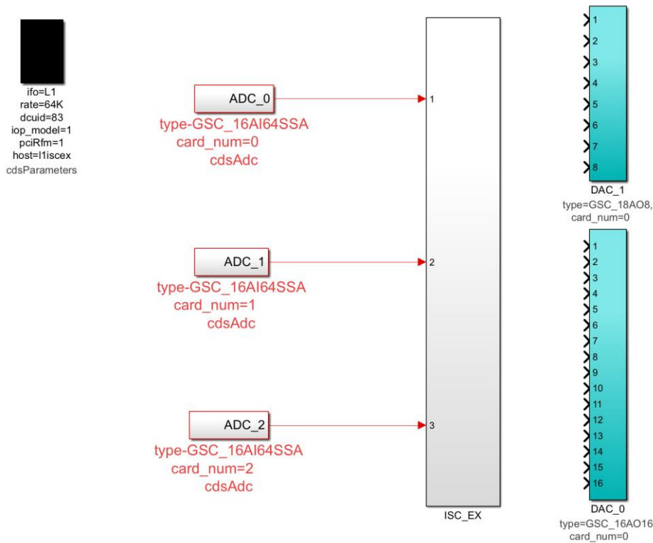
Figure 2: Example IOP Model - Top Level
