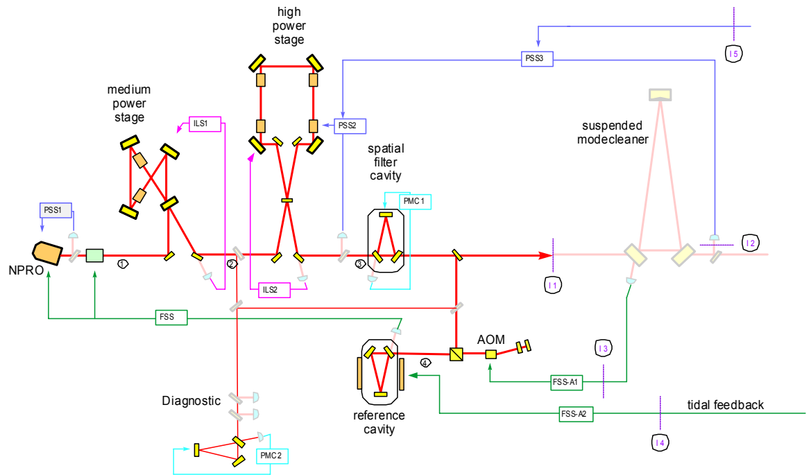
Figure 23. Schematic of the Advanced LIGO PSL.
