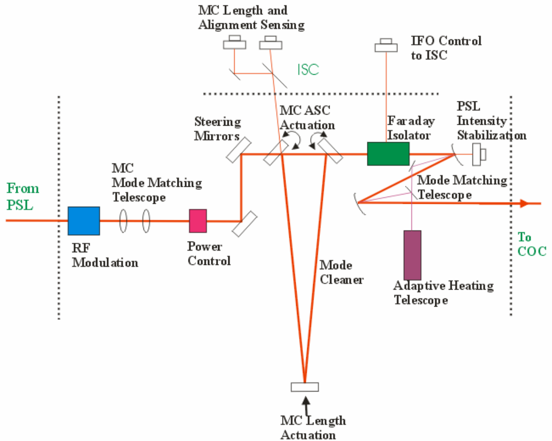
Figure 3 Schematic diagram of the Advanced LIGO Input Optics (IO) subsystem.
