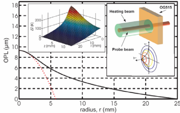
Fig. XX Calculated radial dependence of the optical path difference (OPD) assuming 4 W of heating power in a 7.2 mm diameter beam. The solid line results from an exact solution of the thermal diffusion equation; the dotted line displays the OPD assuming a parabolic lens. Right inset: schematic view of laser adaptive mode control. Left inset: the spatial dependence of the temperature profile \Delta T(r,z) .
