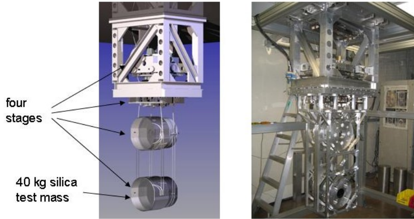
Figure 20. Left: schematic diagram of quadruple suspension showing main chain and parallel reaction chain for interferometer control actuation, with lower support structure removed for clarity. Right: all-metal controls prototype under test at Caltech
