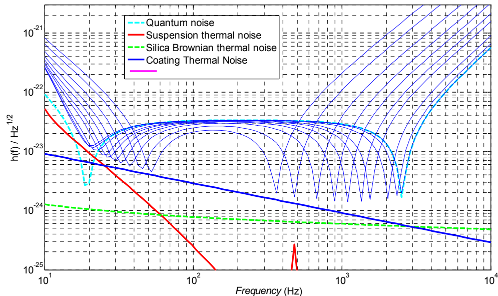
Figure 7 Strain sensitivity curves for a narrowband interferometer. By changing from a signal recycling mirror optimized for broadband operation to one chosen to give optimum performance around 800 Hz, good performance at a selected frequency between ~400–2000 Hz can be achieved by tuning the signal mirror position microscopically; the set of curves shown span a mirror motion of less than a micron. At the lower end of the range, coating thermal noise limits the performance; at higher frequencies, above ~500 Hz, the quantum noise limits the best performance (modeled using Bench 23 )
