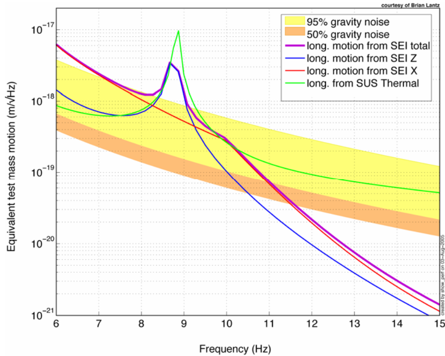
Figure 1 Predicted test mass displacement noise. The orange and yellow shaded regions are the expected longitudinal (beam direction) motion from direct gravity coupling, at 50 th and 95 th percentile ground motion measured at the LIGO sites; this dominates over the seismic noise above 11 Hz or so. The red, blue and purple lines are, respectively, the contributions to test mass motion from horizontal and vertical seismic isolation system motion and the total seismic contribution at about the 90 th percentile level. The green curve is the expected suspension (pendulum) thermal noise; it exceeds the seismic noise above about 10.3 Hz.
