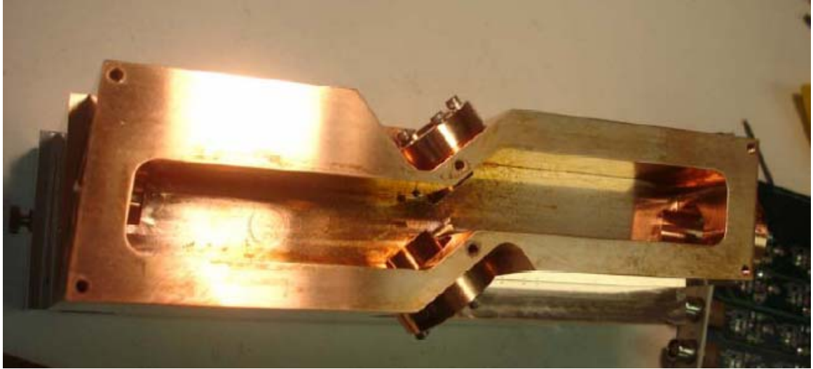
Figure 8: the 4-mirror output mode cleaner prototype at the Caltech 40-meter prototype interferometer.
