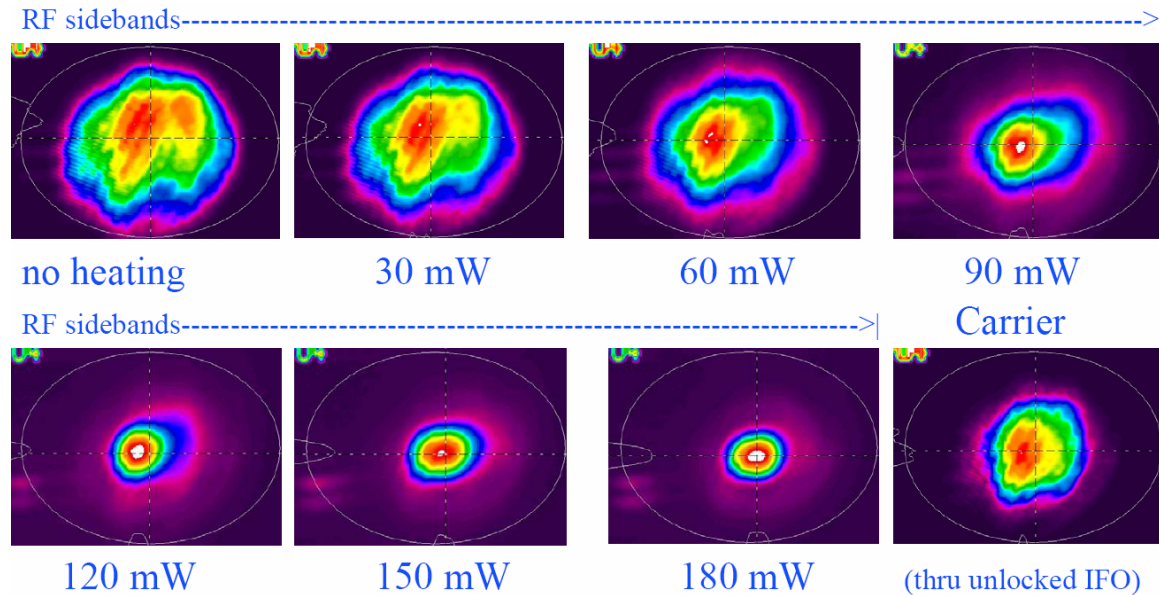
Figure 6: RF sideband mode shape control using thermal compensation. Note the optimum overlap between RF sideband and carrier mode at 90 mW heating power.
