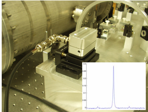
Fig. XX- The Advanced LIGO electro-optic modulators with modulated spectrum shown in the inset.
