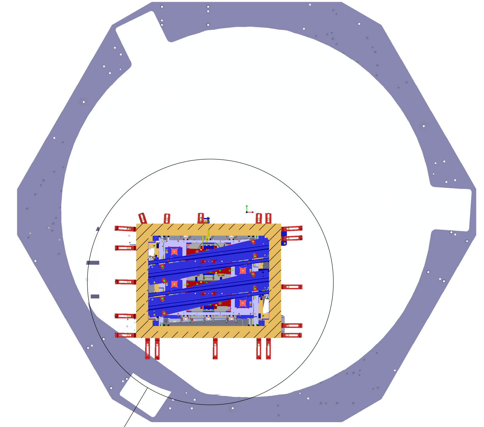
TOP VIEW (LOOKING DOWN)
