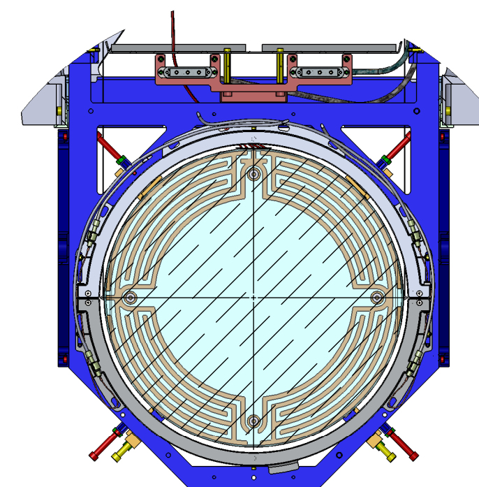
SECTION C-C (RING HEATER CLOSED) SCALE: ENLARGED
