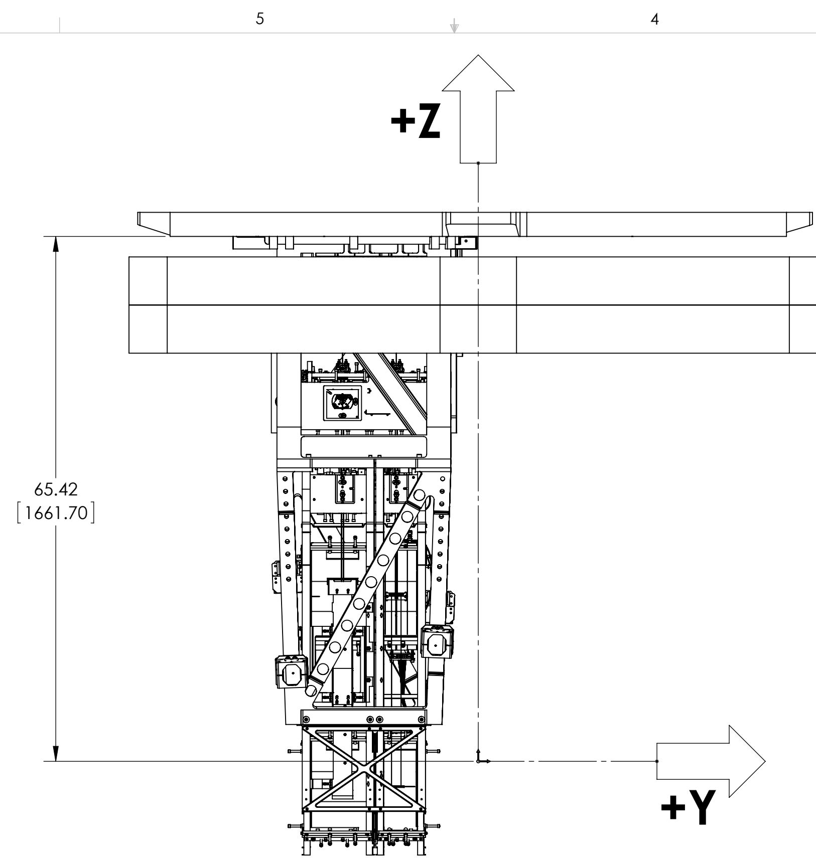
RIGHT VIEW
