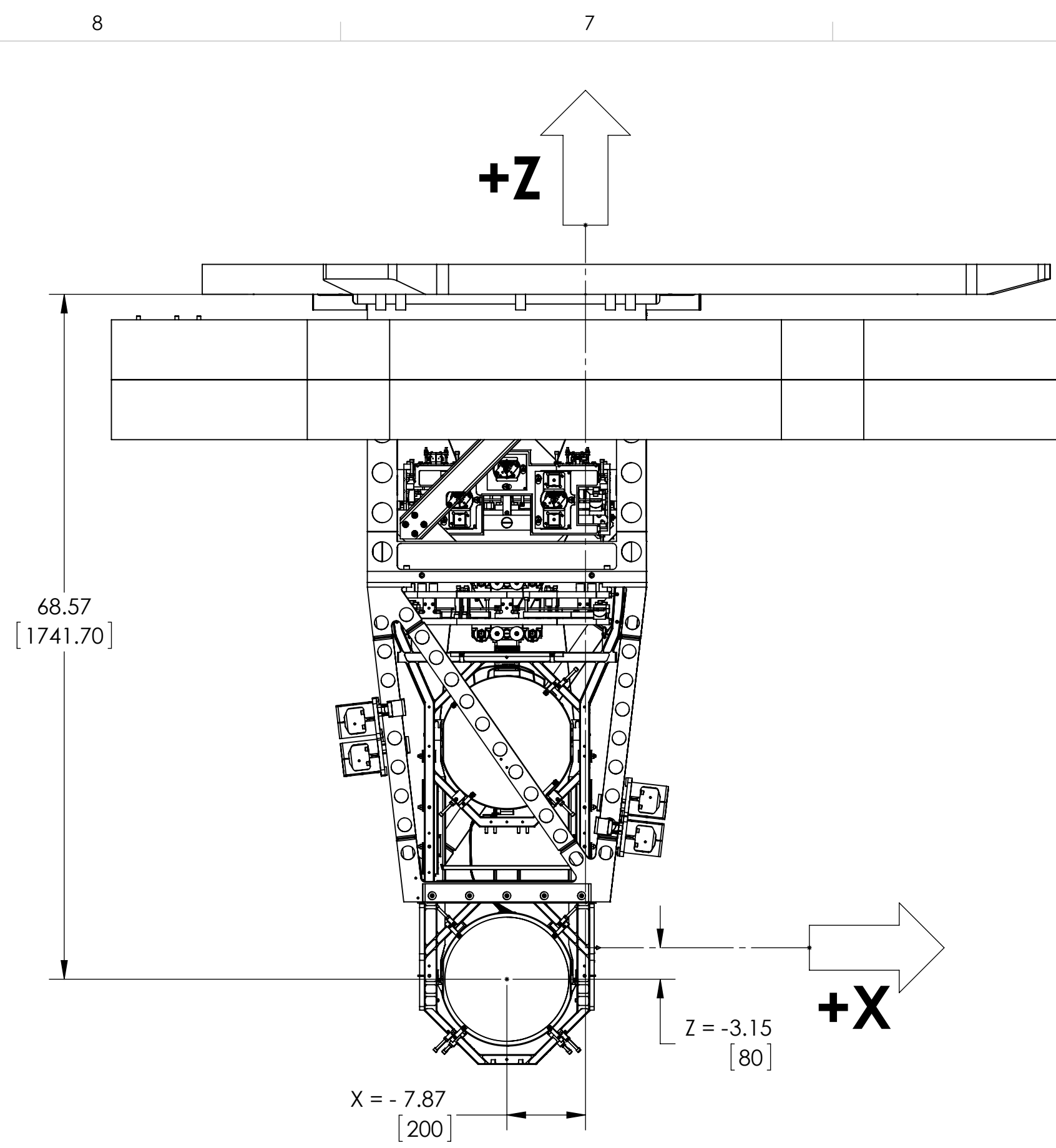
FRONT VIEW
