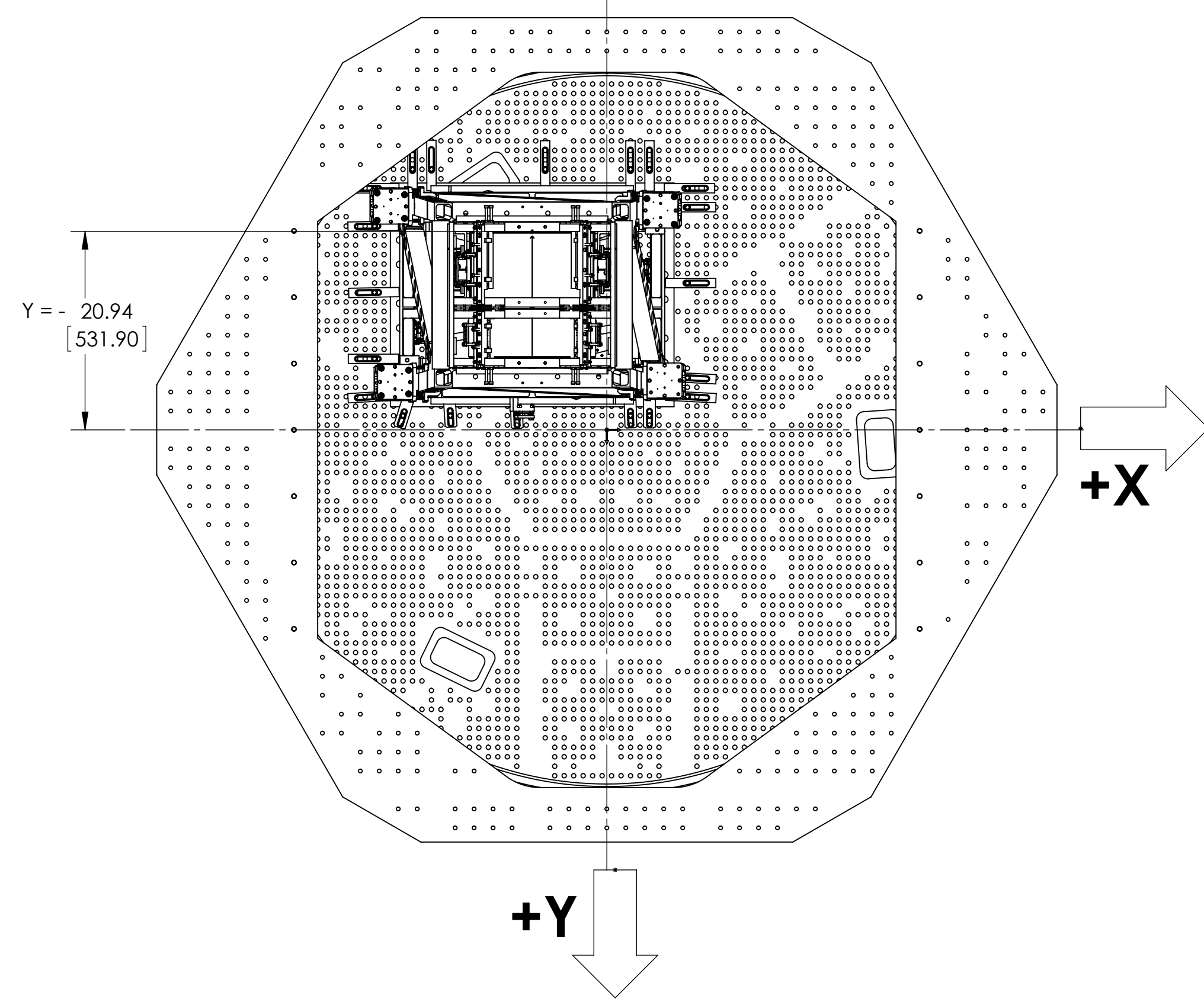
BOTTOM VIEW (LOOKING UP)
