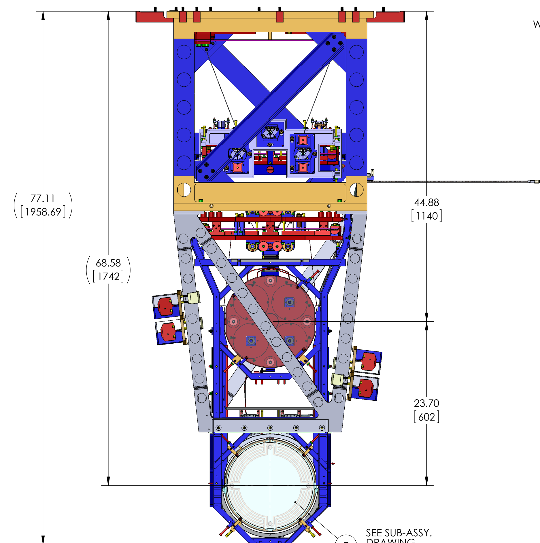
SECTION C-C (RING HEATER OPEN) SCALE: ENLARGED
