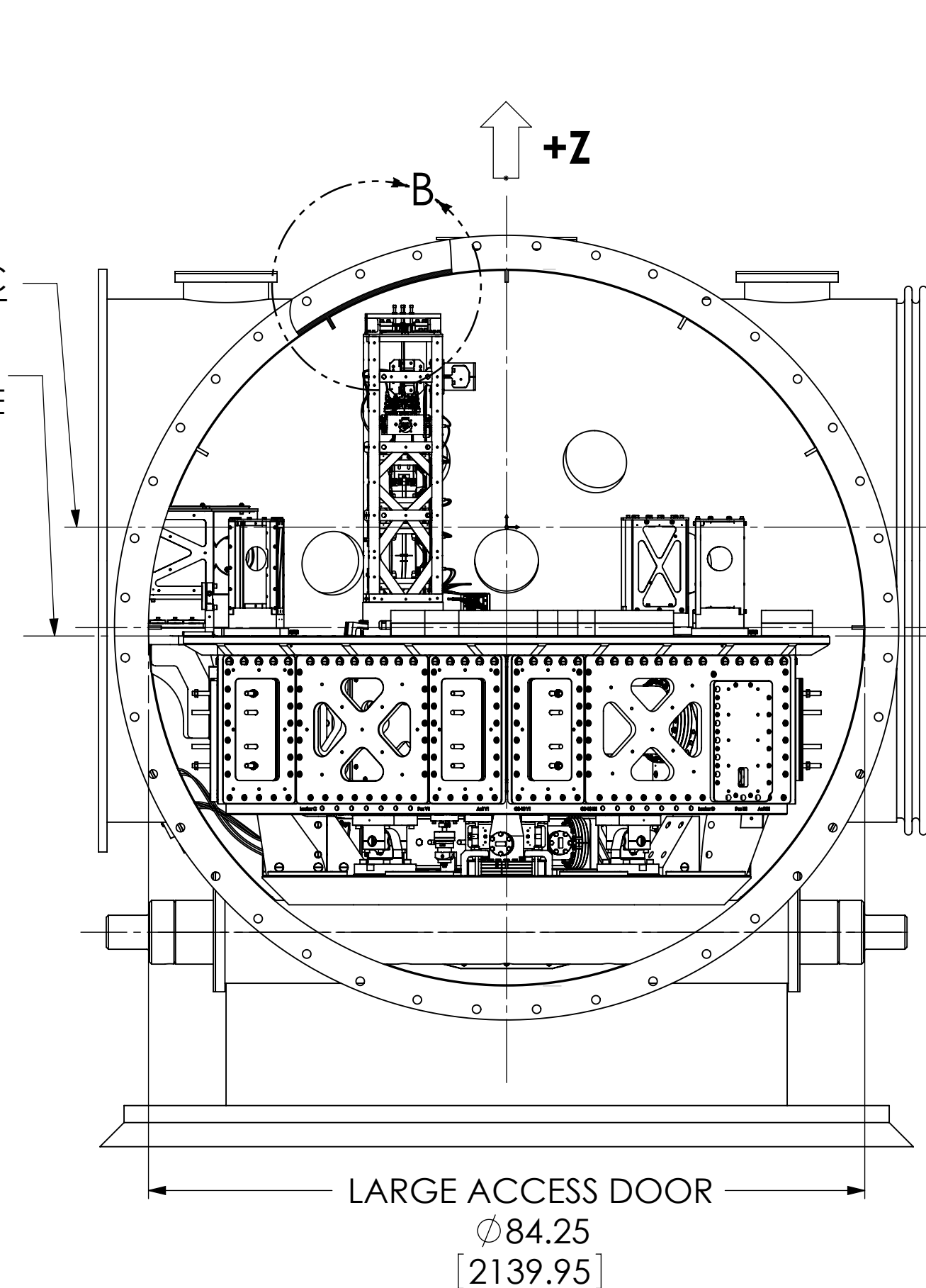
RIGHT VIEW
