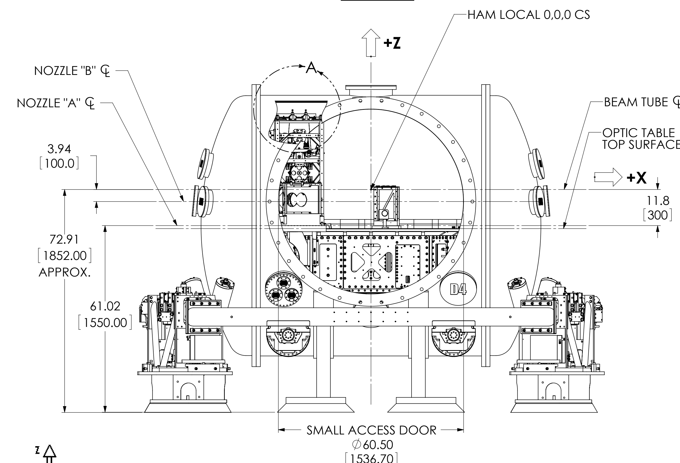
FRONT VIEW
