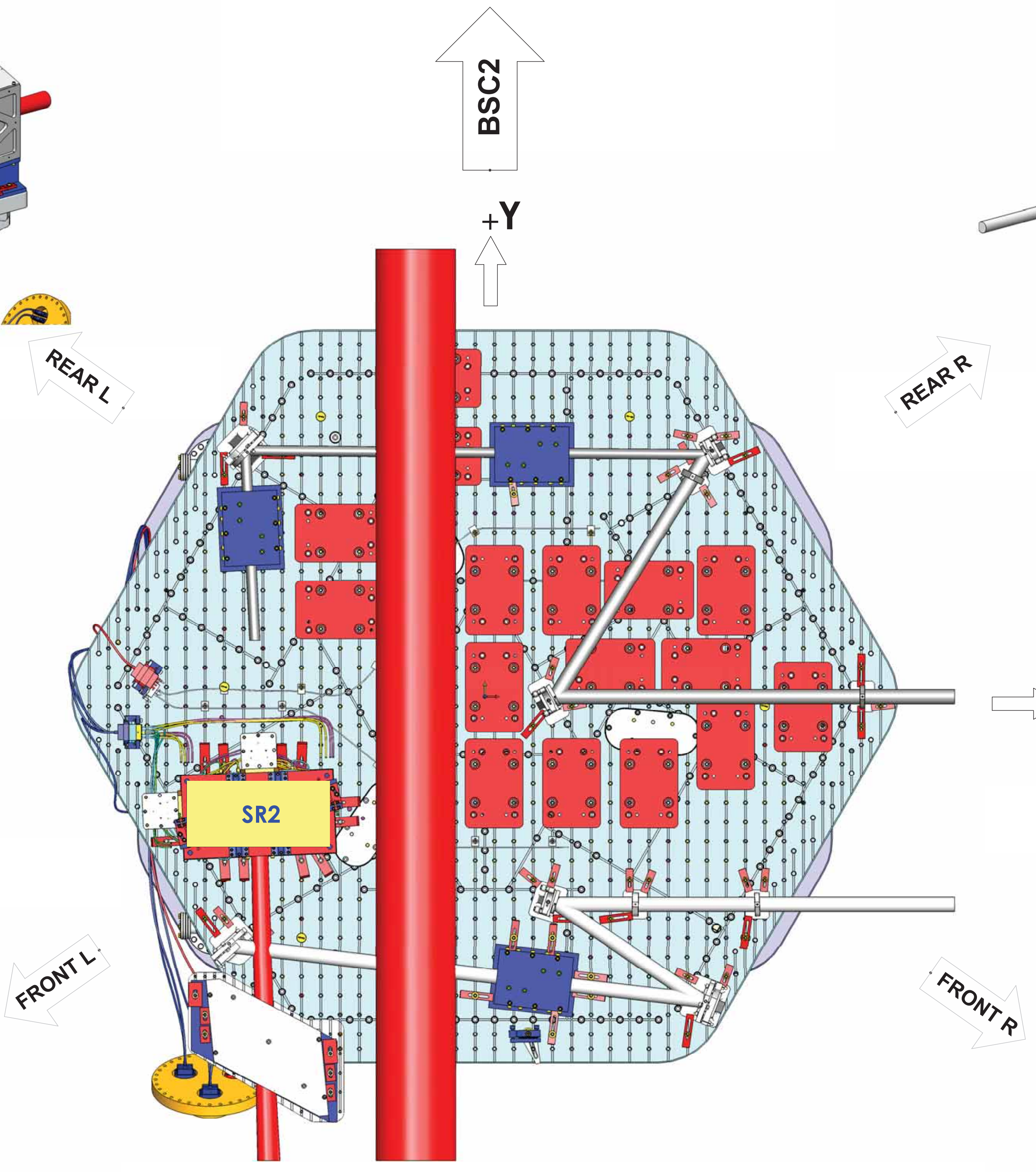
TOP VIEW
