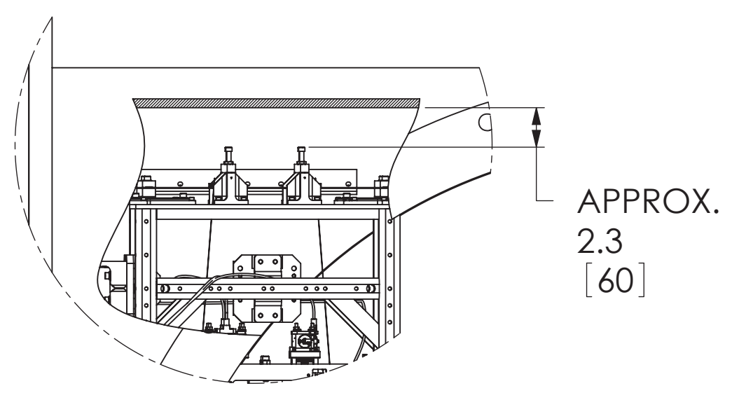
DETAIL A SCALE 1:8
