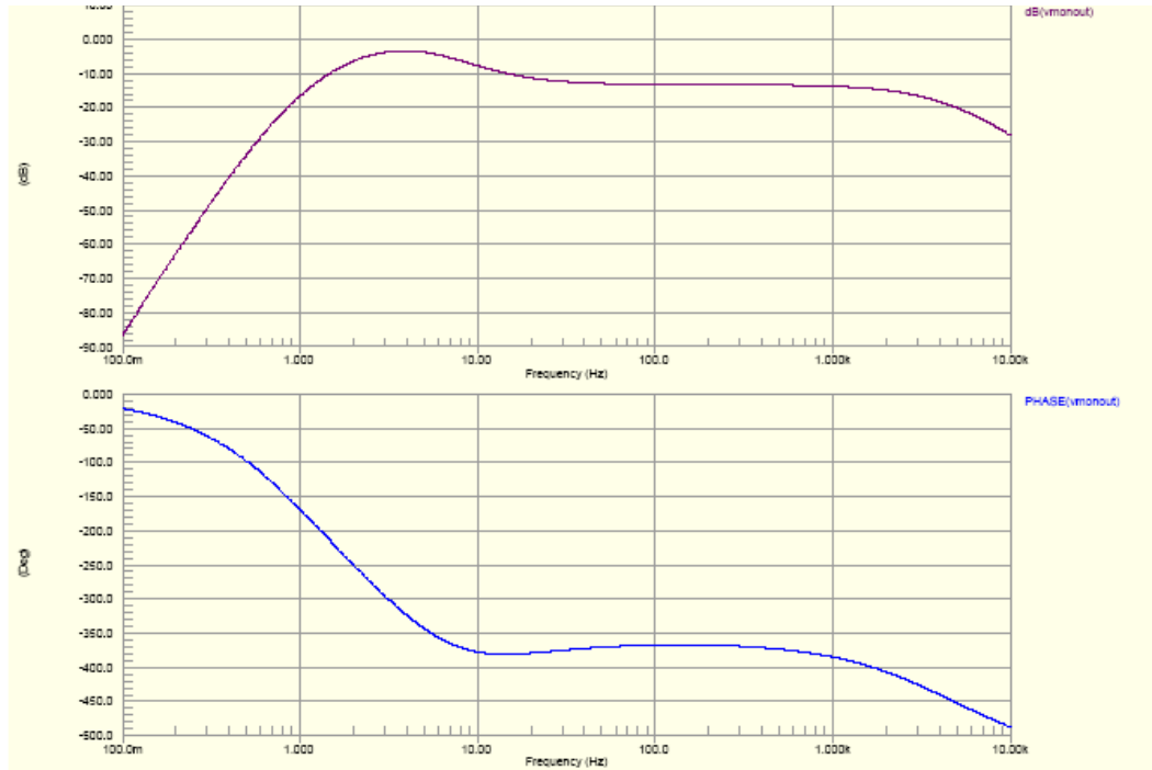
Figure 4: Transfer Function from Input to Noise Monitor Output (Low Noise Mode)
