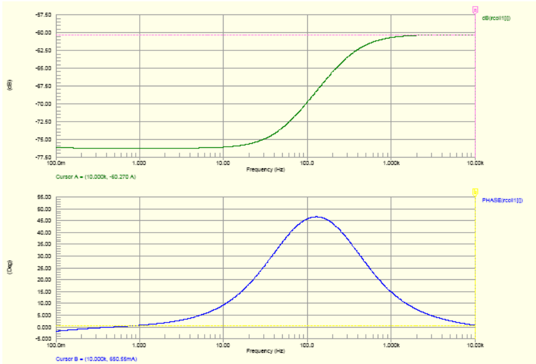
Figure 1: High Dynamic Range Transfer Function
