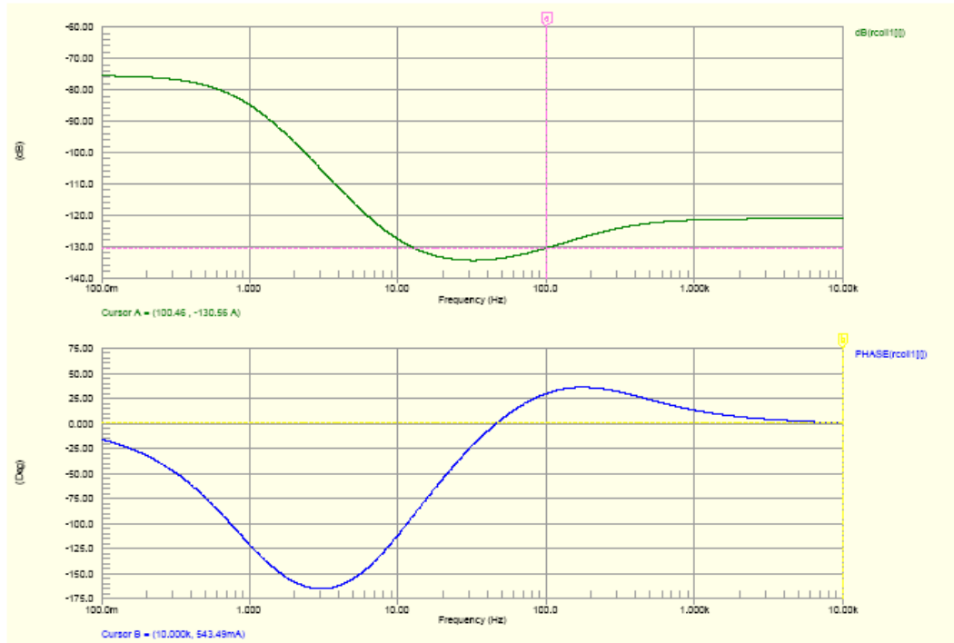
Figure 2: Low Noise Transfer Function
