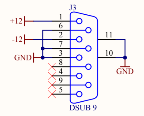
To the Pre Amplifier2
